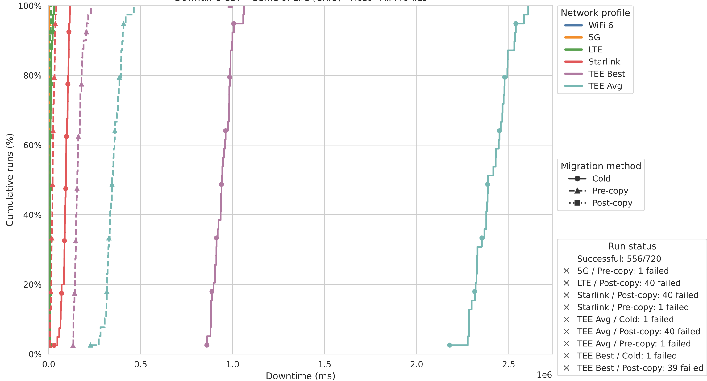
Downtime CDF - Game of Life (CRIU) - Host - All Profiles
