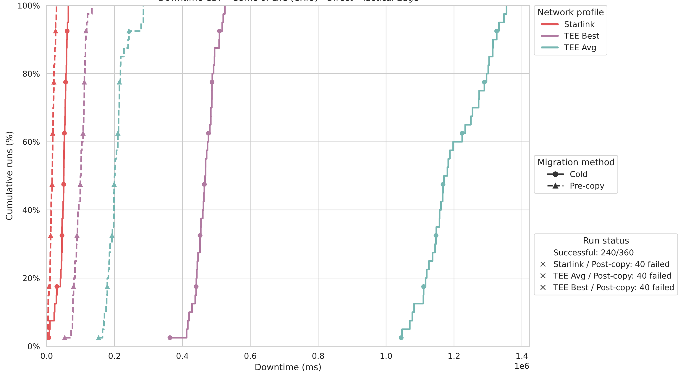
Downtime CDF - Game of Life (CRIU) - Direct - Tactical Edge
