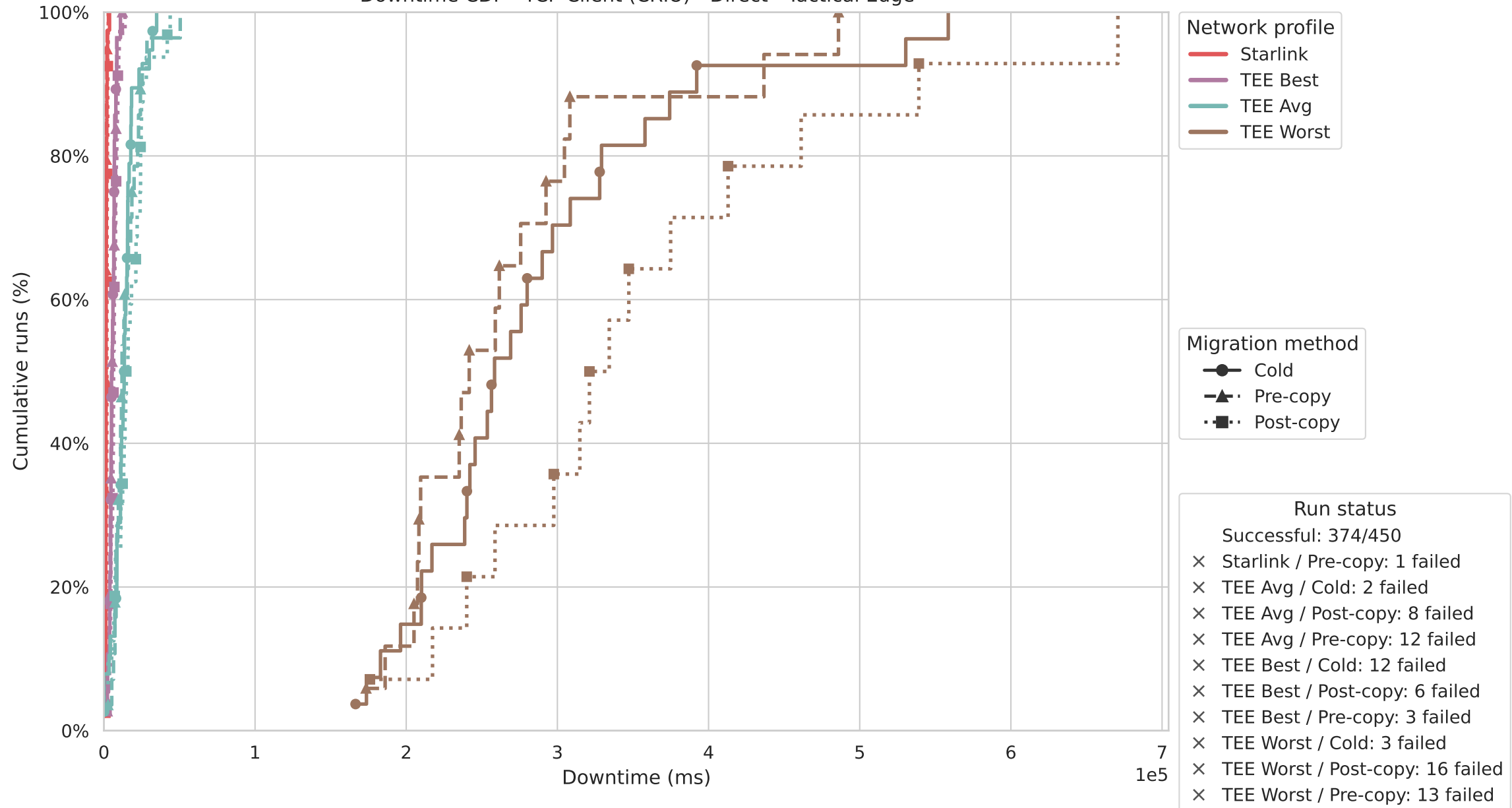
Downtime CDF - TCP Client (CRIU) - Direct - Tactical Edge
