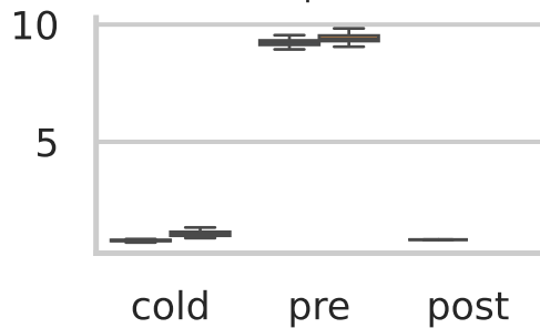
Source | CPU (%)
