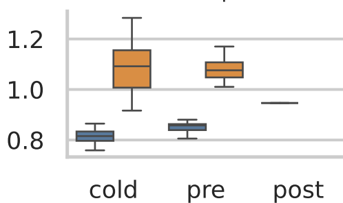
Destination | CPU (%)
