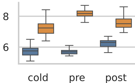
Source | CPU (%)
