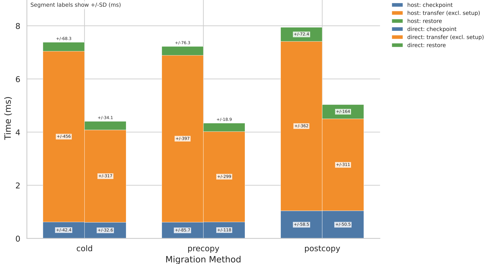
Migration Phase Breakdown (Mean) - 4_Starlink
