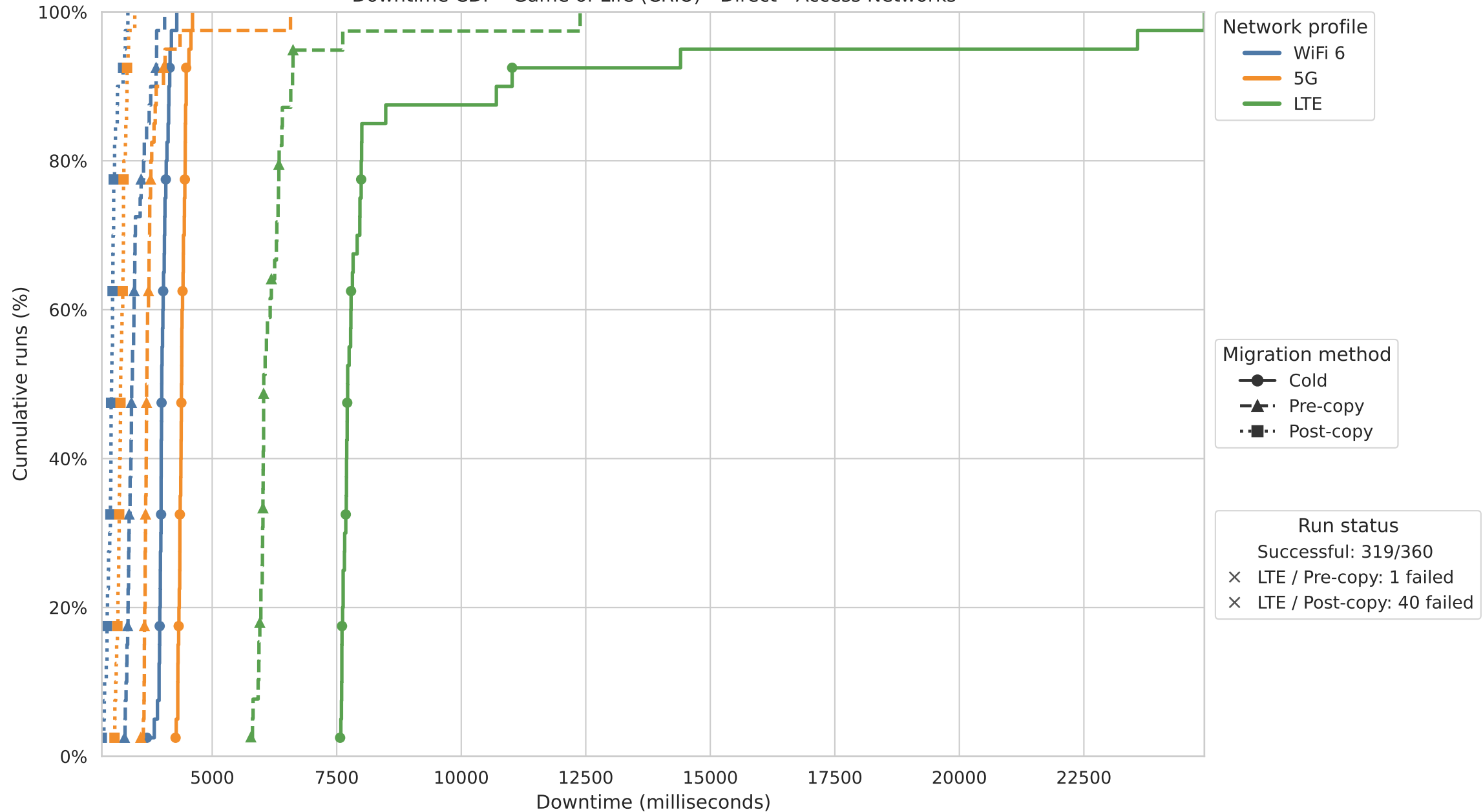
Downtime CDF - Game of Life (CRIU) - Direct - Access Networks
