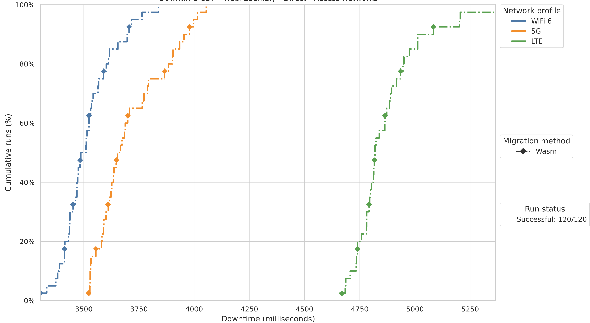
Downtime CDF - WebAssembly - Direct - Access Networks
