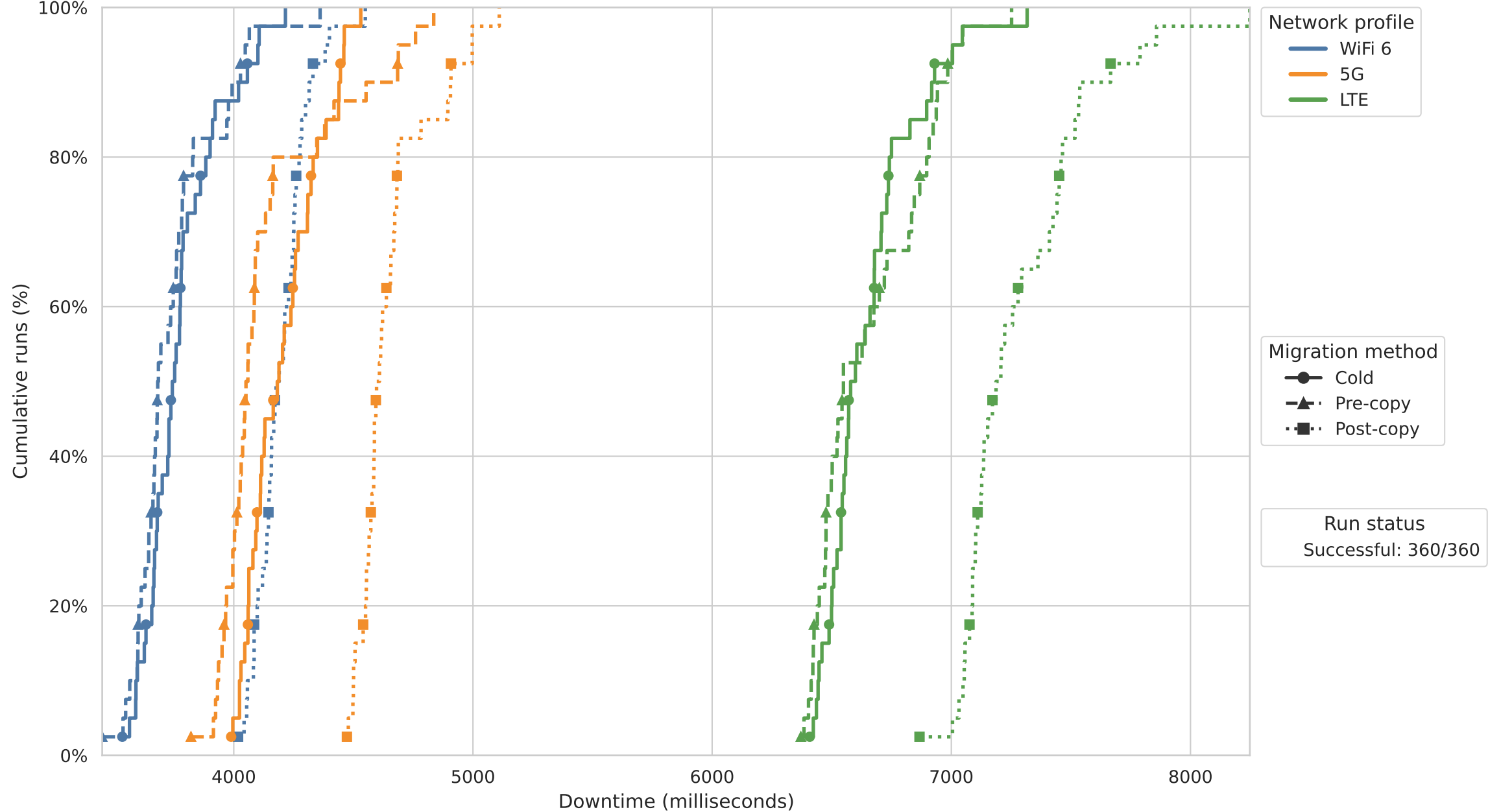
Downtime CDF - Counter (CRIU) - Host - Access Networks
