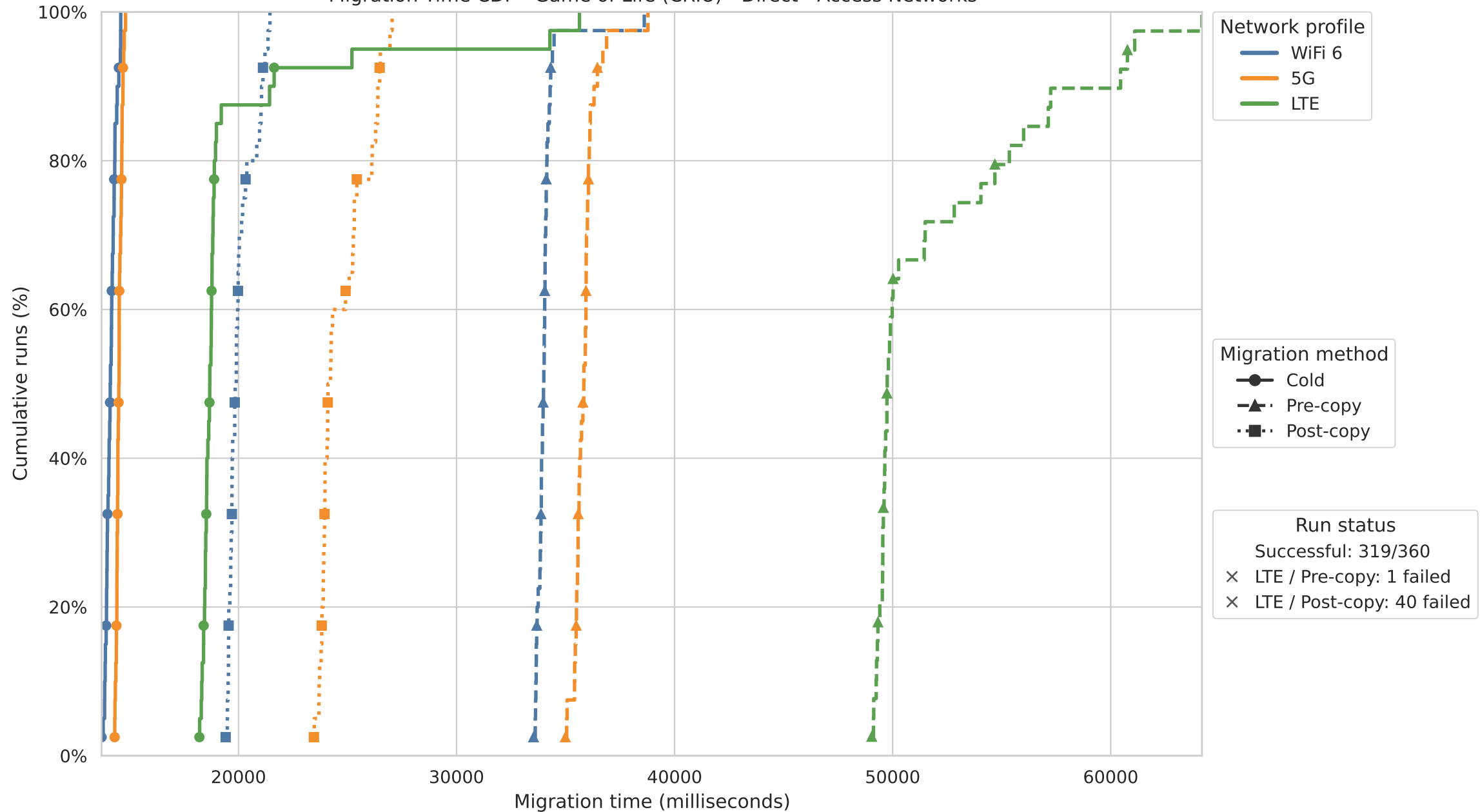
Migration Time CDF - Game of Life (CRIU) - Direct - Access Networks
