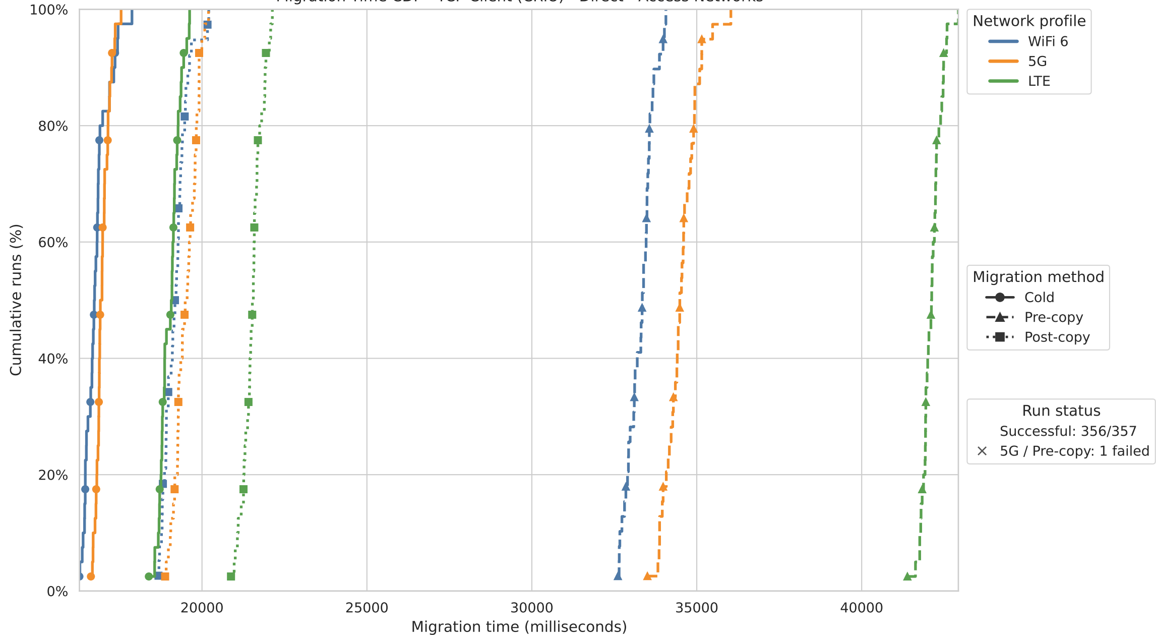
Migration Time CDF - TCP Client (CRIU) - Direct - Access Networks
