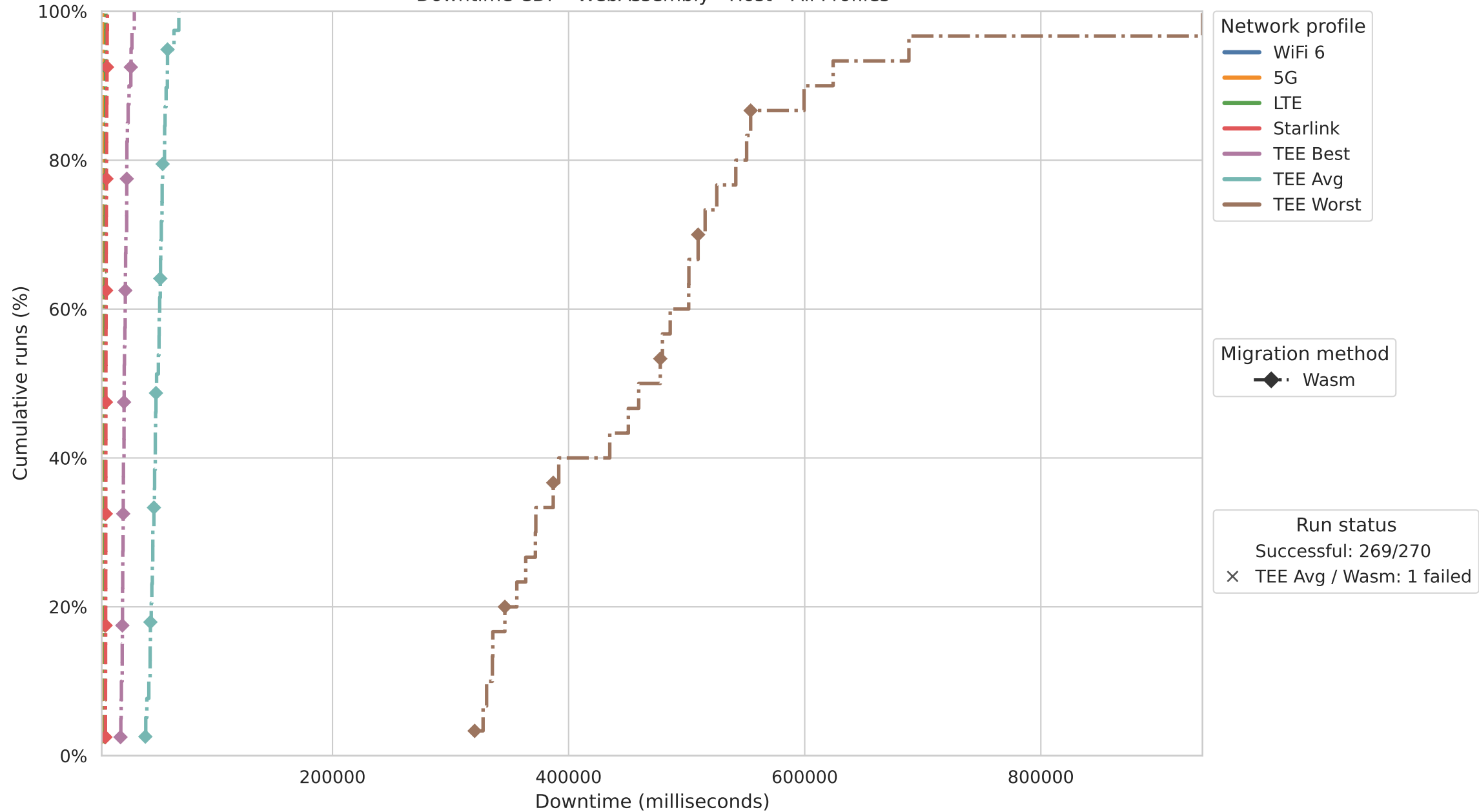
Downtime CDF - WebAssembly - Host - All Profiles
