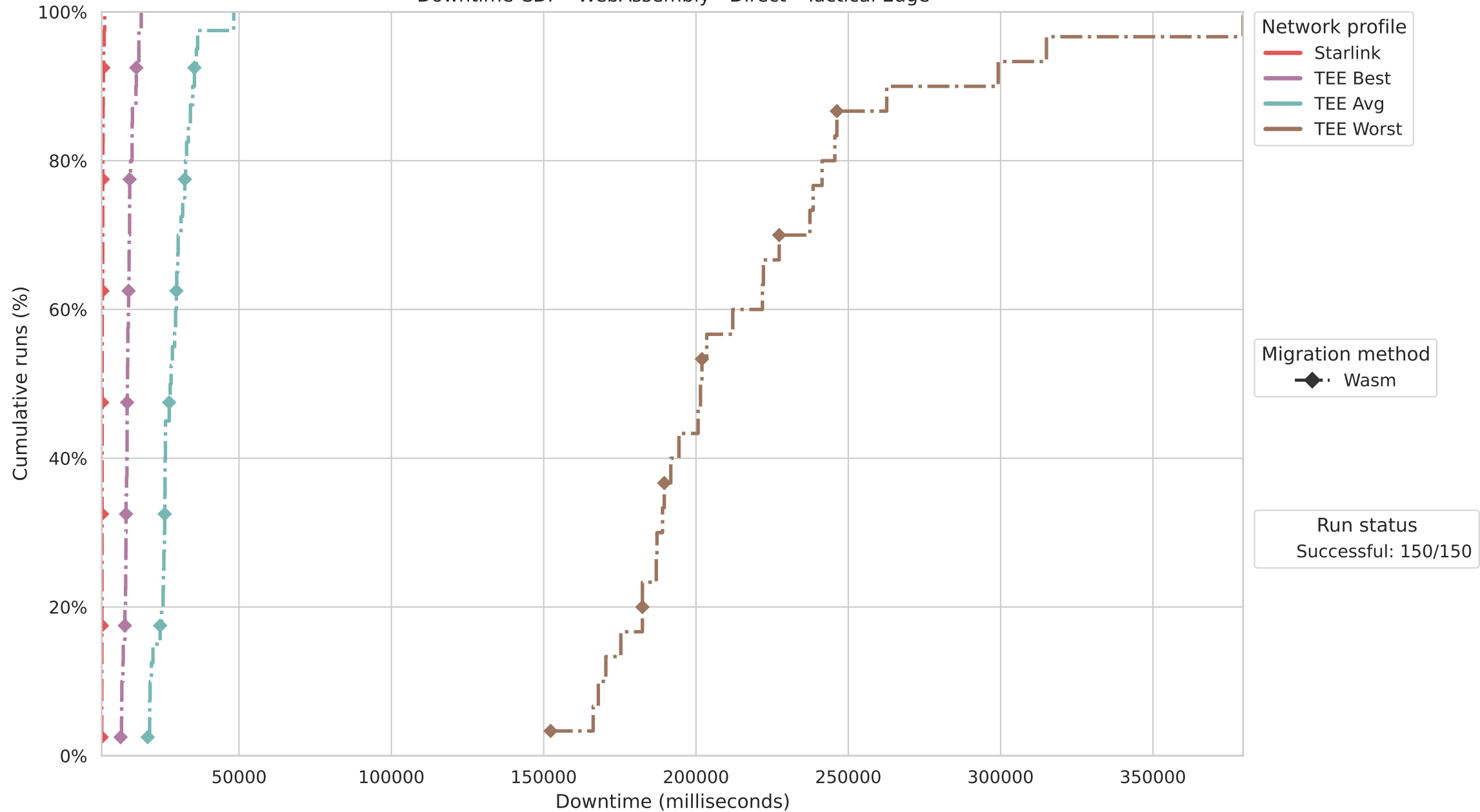
Downtime CDF - WebAssembly - Direct - Tactical Edge
