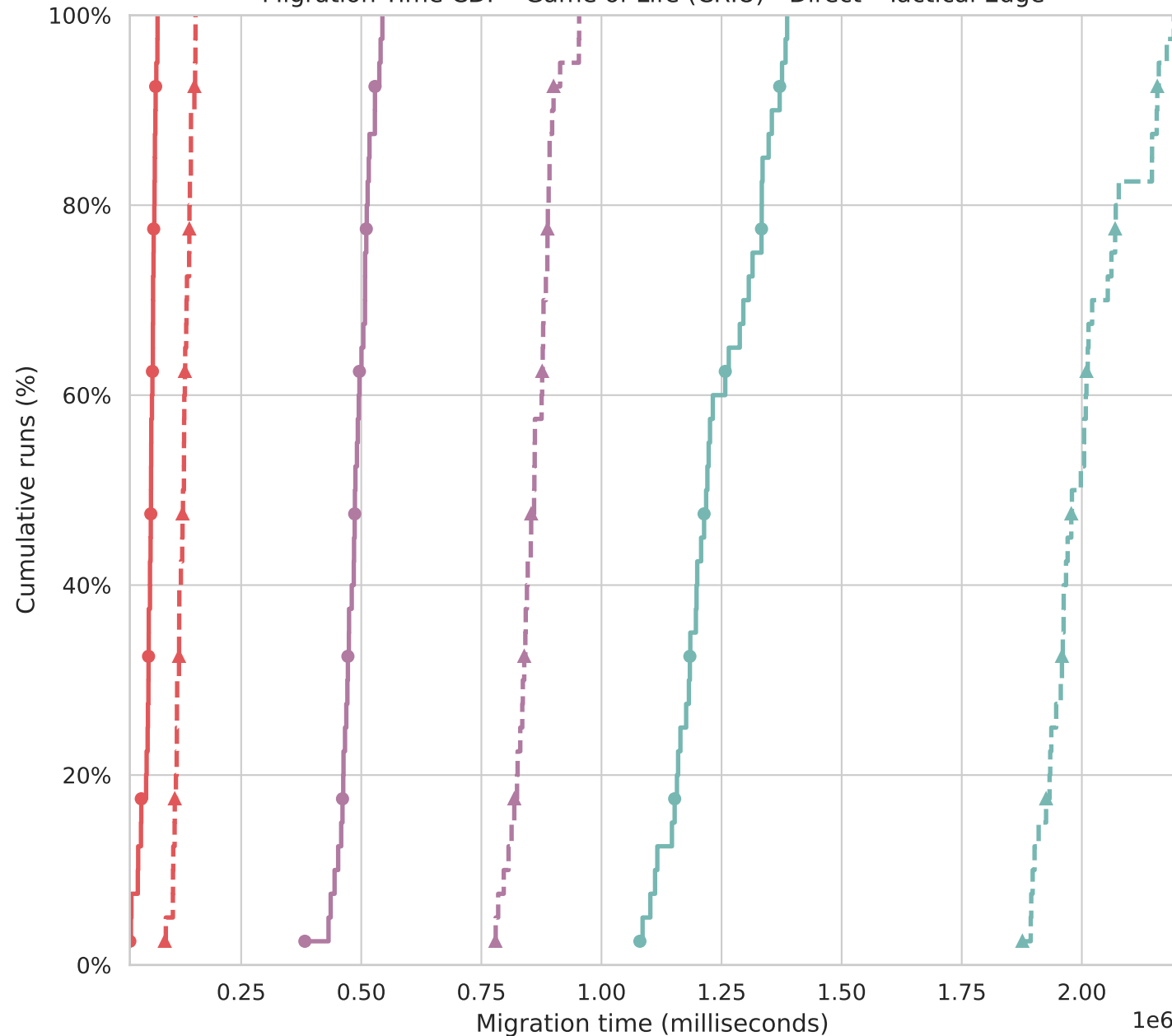
Migration Time CDF - Game of Life (CRIU) - Direct - Tactical Edge
