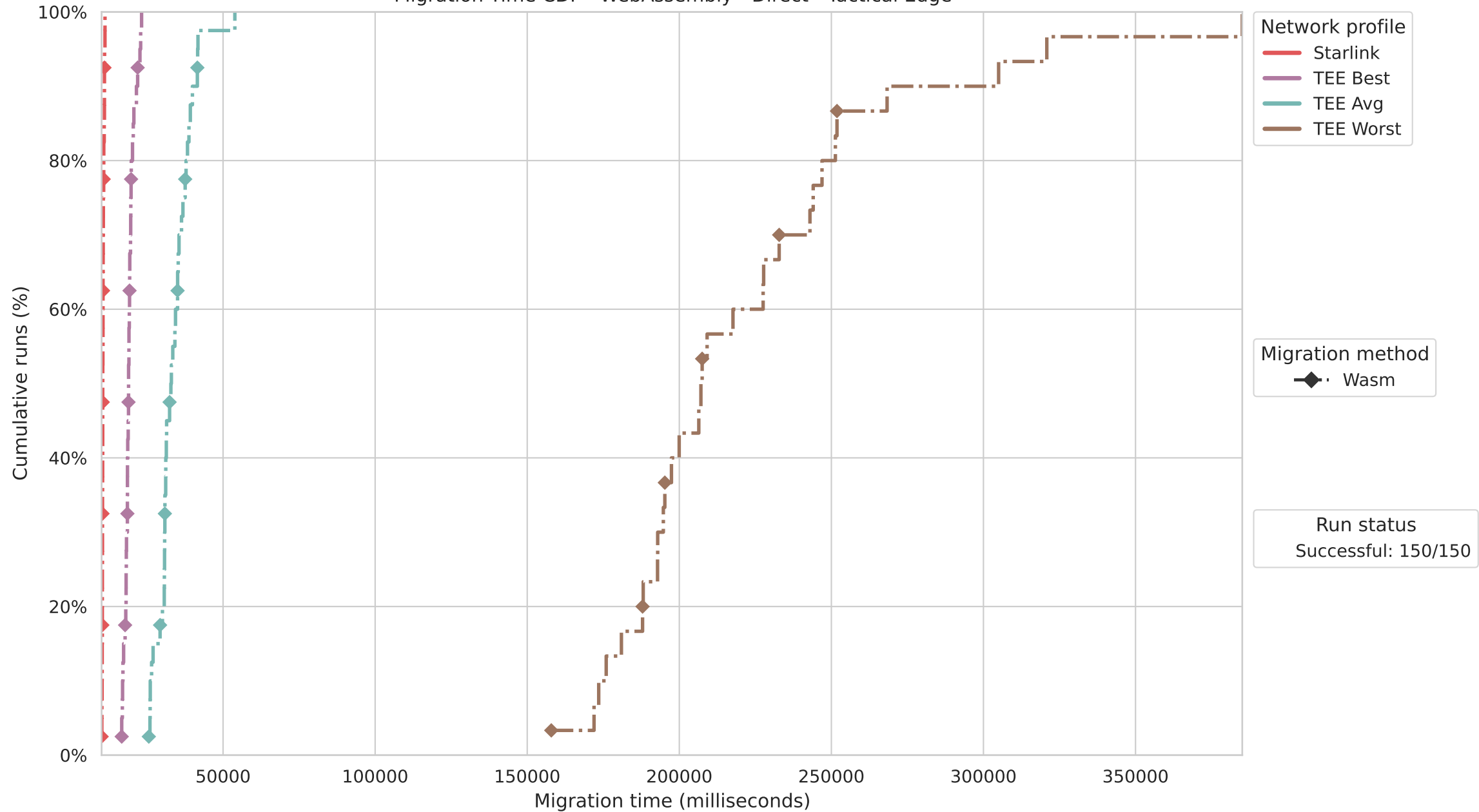
Migration Time CDF - WebAssembly - Direct - Tactical Edge
