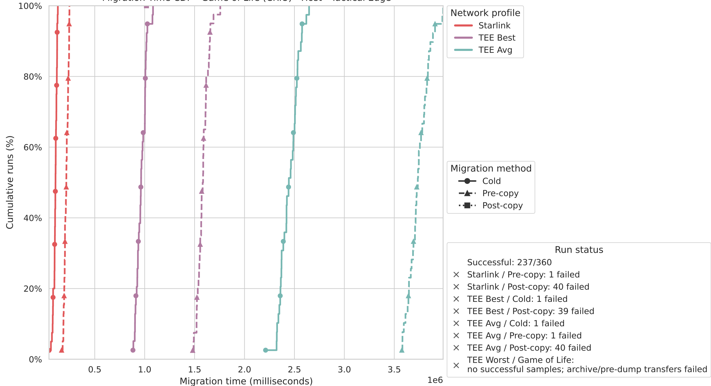
Migration Time CDF - Game of Life (CRIU) - Host - Tactical Edge
