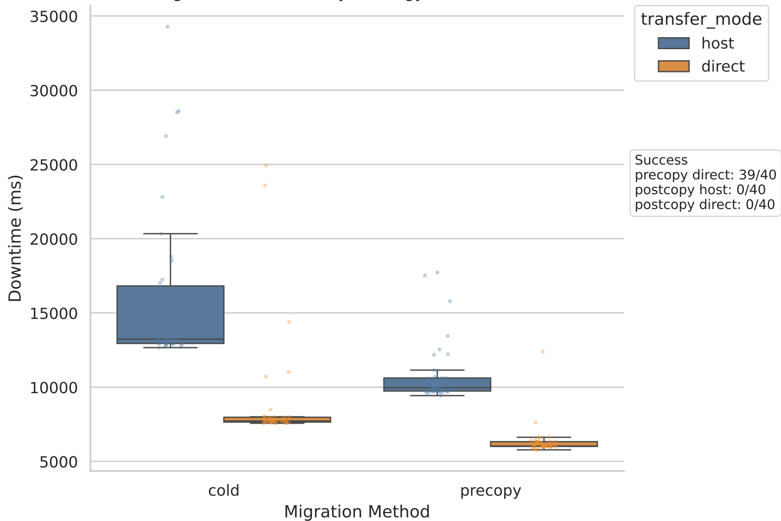
Migration Downtime by Strategy (Host vs Direct)
