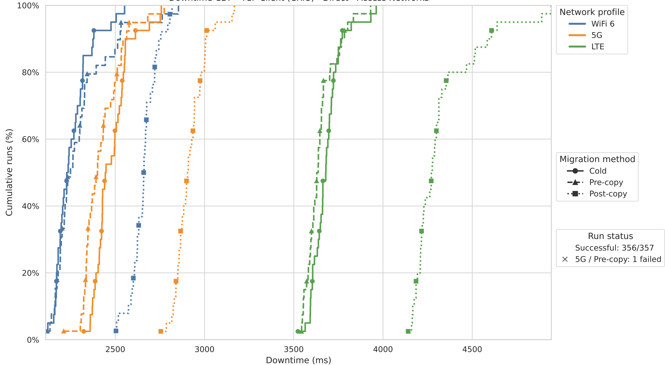
Downtime CDF - TCP Client (CRIU) - Direct - Access Networks
