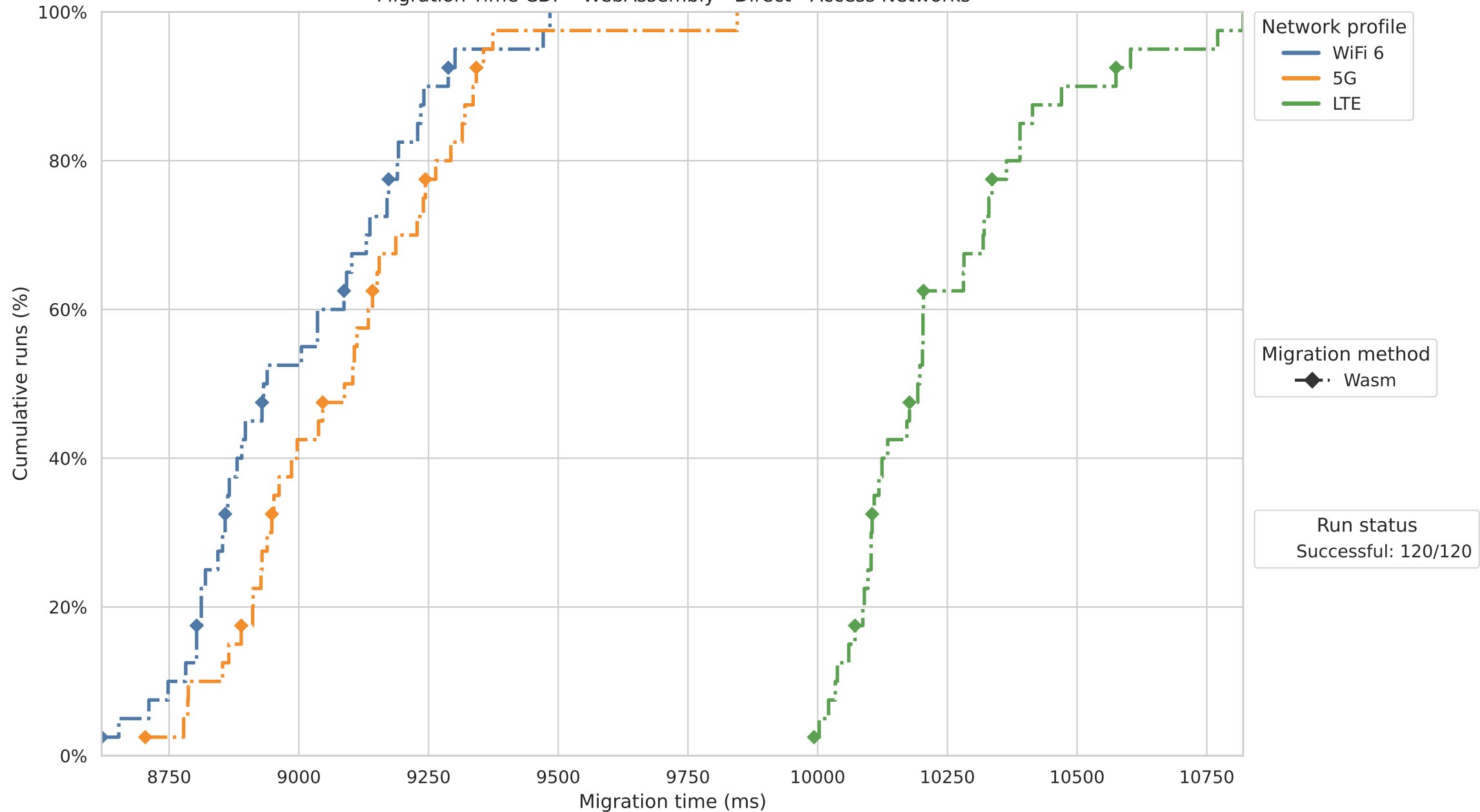
Migration Time CDF - WebAssembly - Direct - Access Networks
