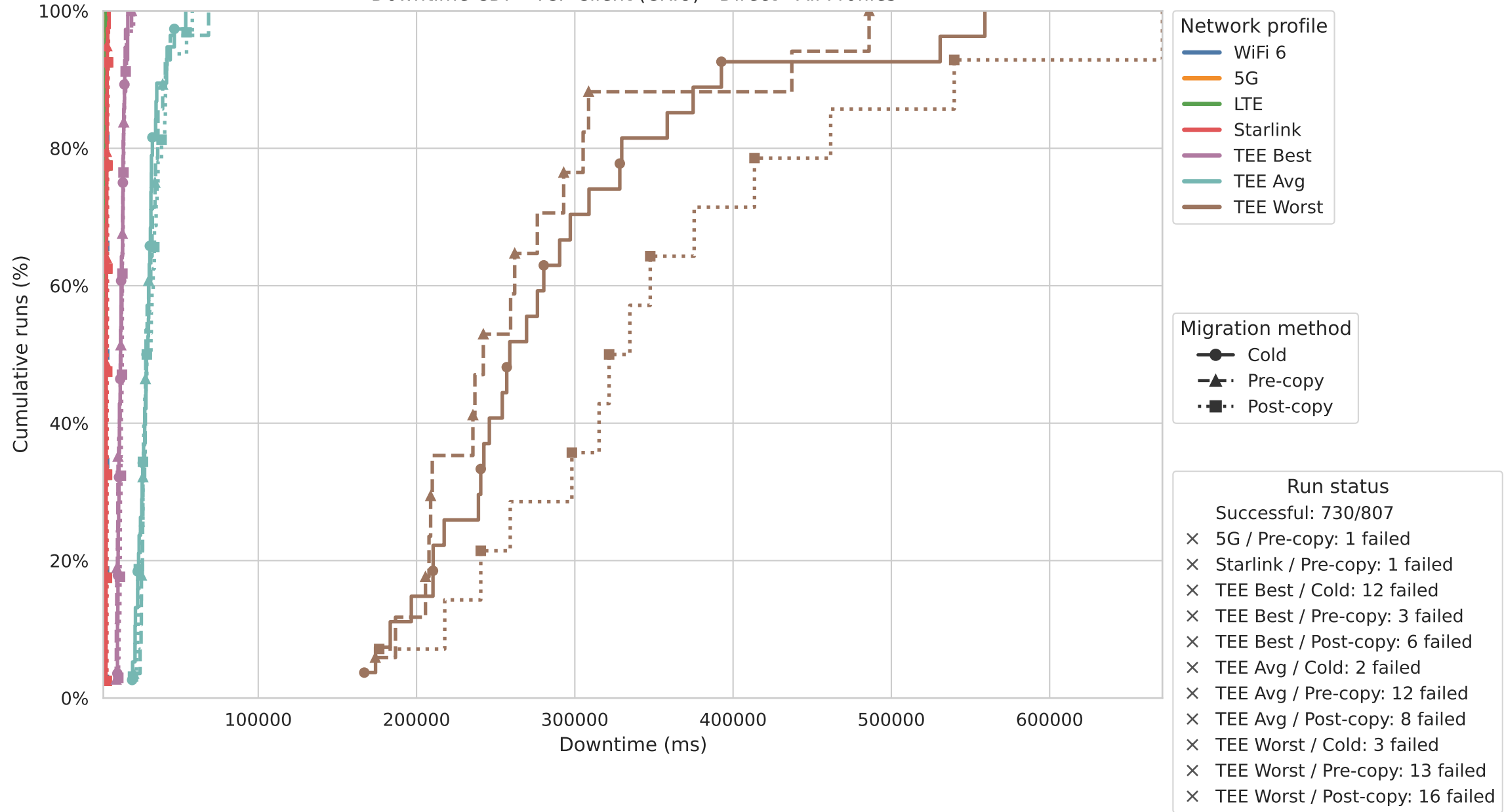
Downtime CDF - TCP Client (CRIU) - Direct - All Profiles
