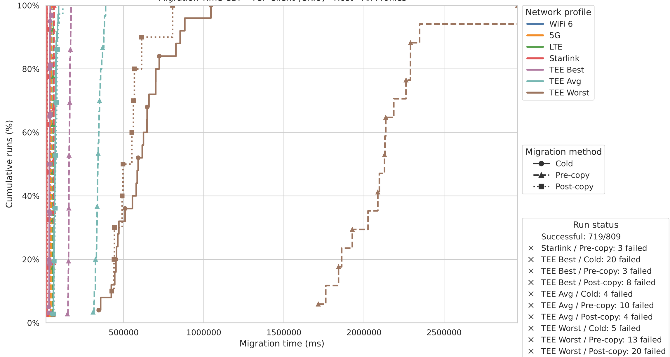
Migration Time CDF - TCP Client (CRIU) - Host - All Profiles
