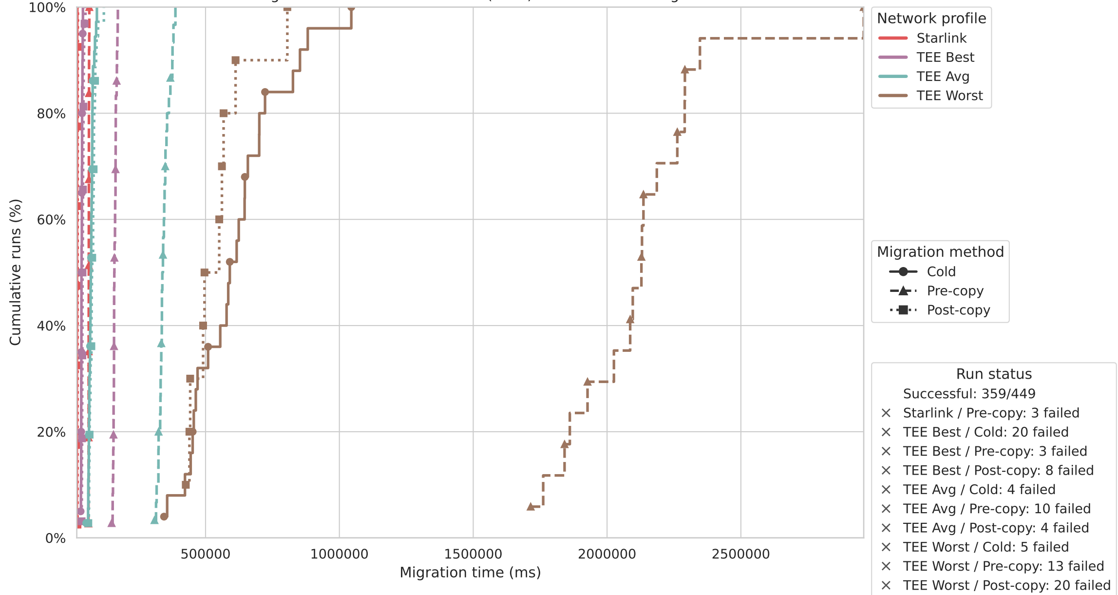
Migration Time CDF - TCP Client (CRIU) - Host - Tactical Edge
