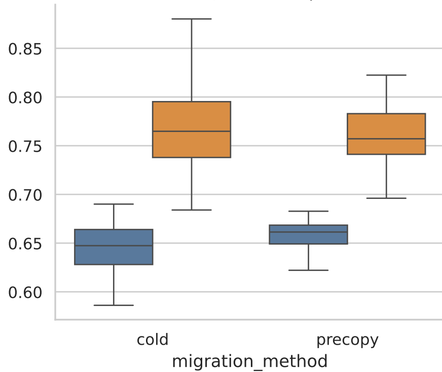
Destination (edge-node-2) | CPU util (%)
