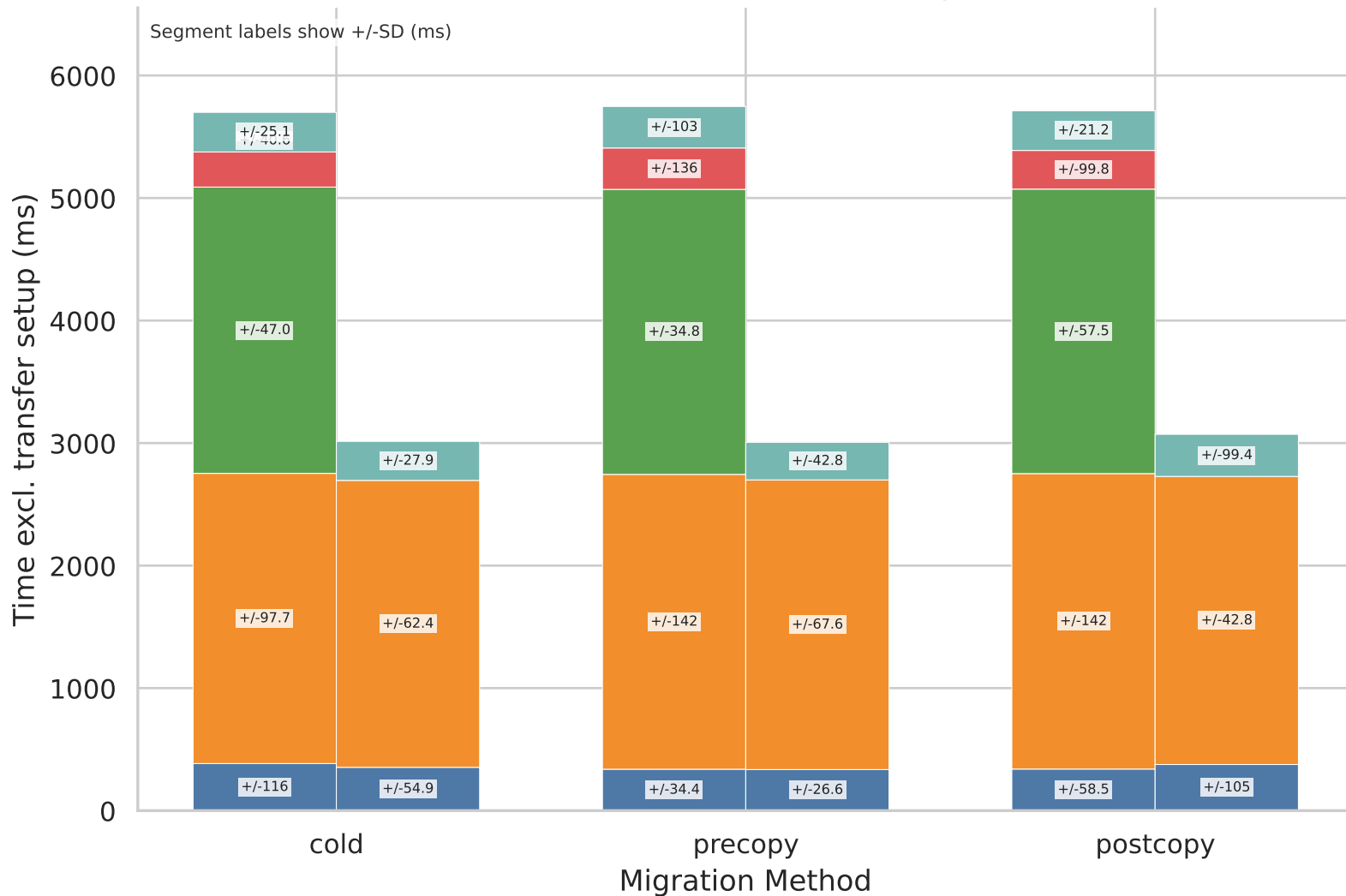
Transfer Phase Breakdown (Mean, setup excluded)
