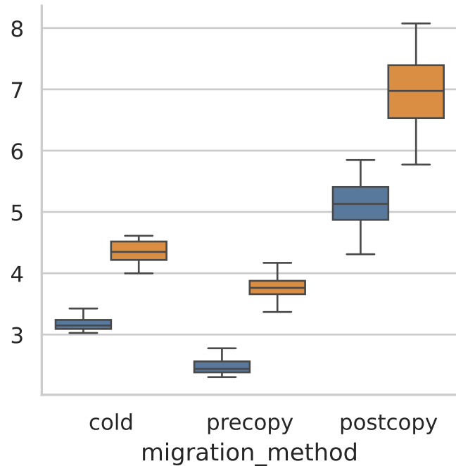
CPU util avg (%)
