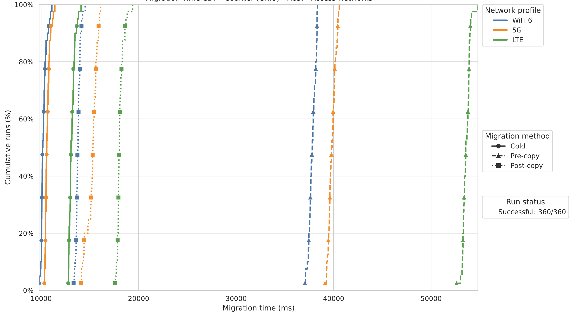
Migration Time CDF - Counter (CRIU) - Host - Access Networks
