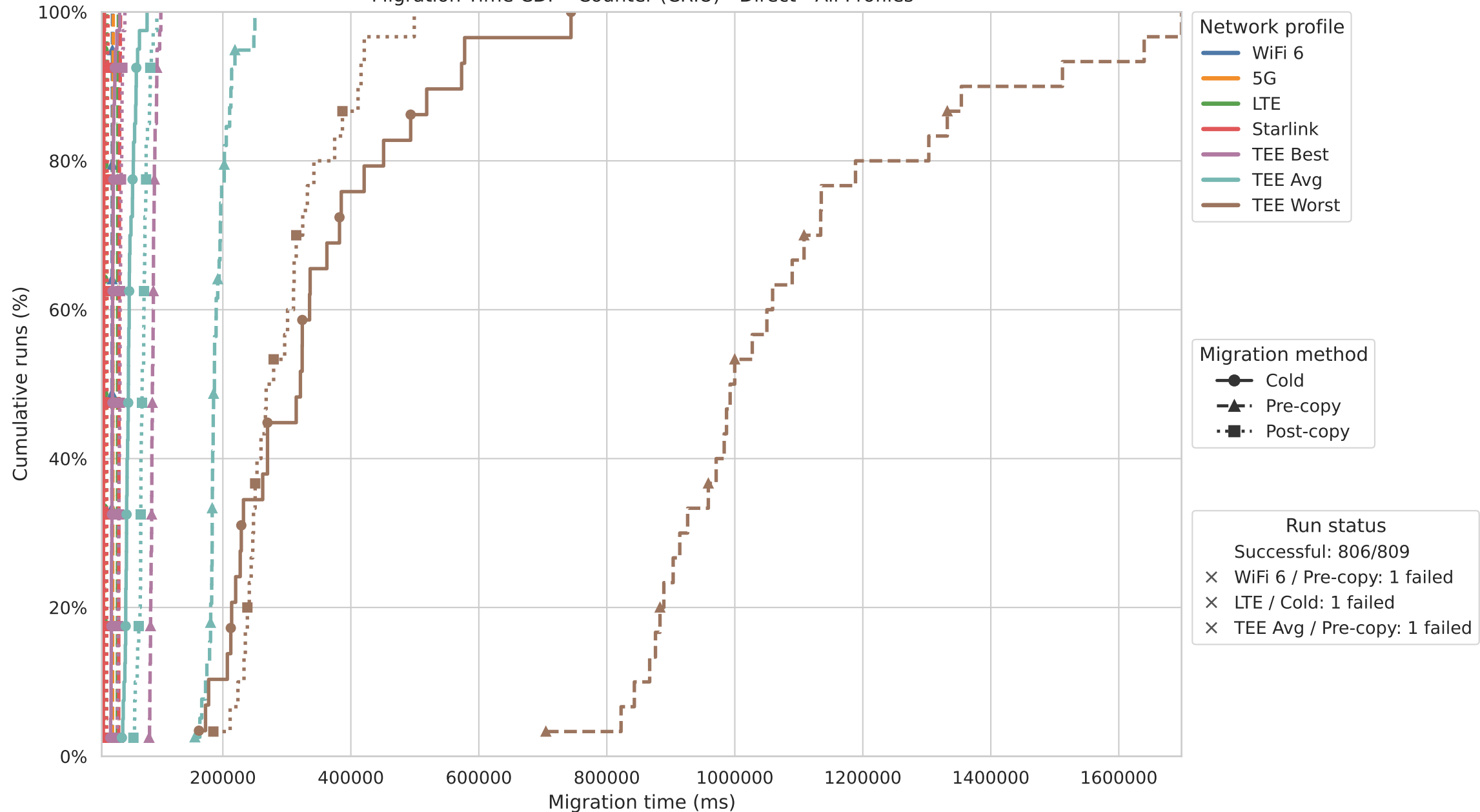
Migration Time CDF - Counter (CRIU) - Direct - All Profiles
