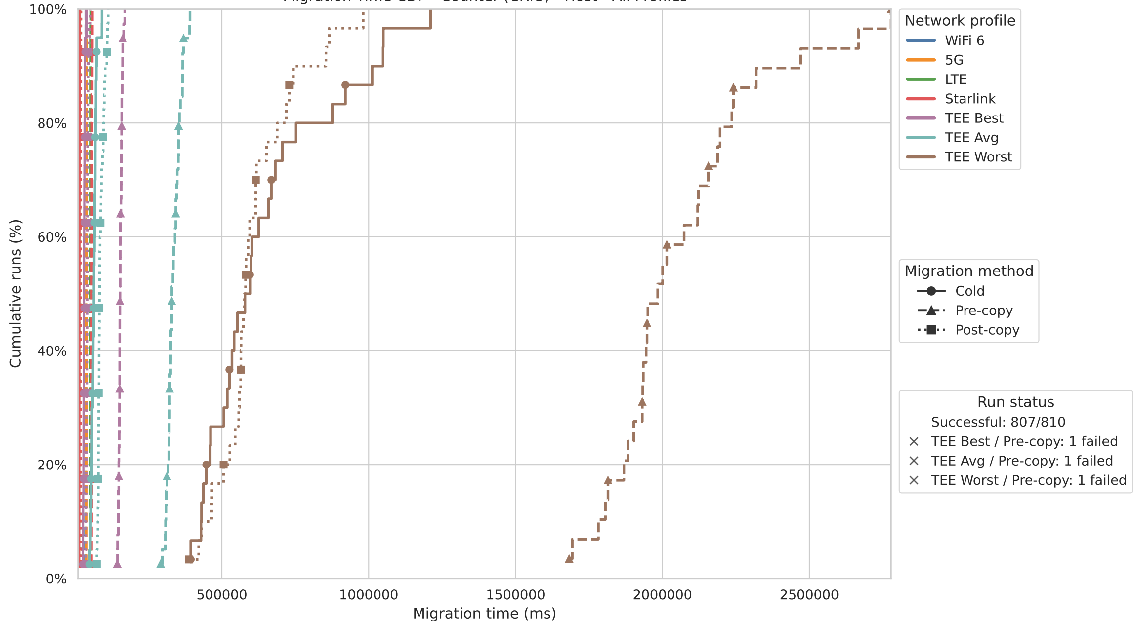
Migration Time CDF - Counter (CRIU) - Host - All Profiles
