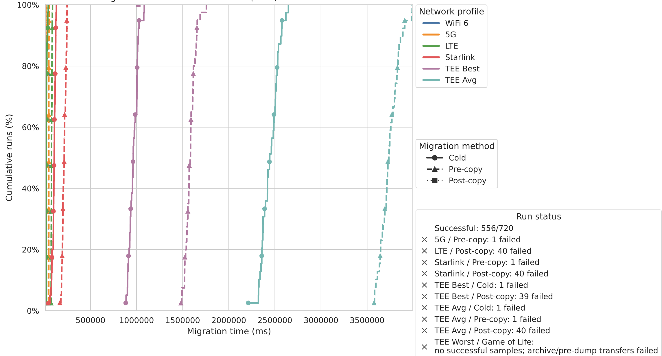
Migration Time CDF - Game of Life (CRIU) - Host - All Profiles
