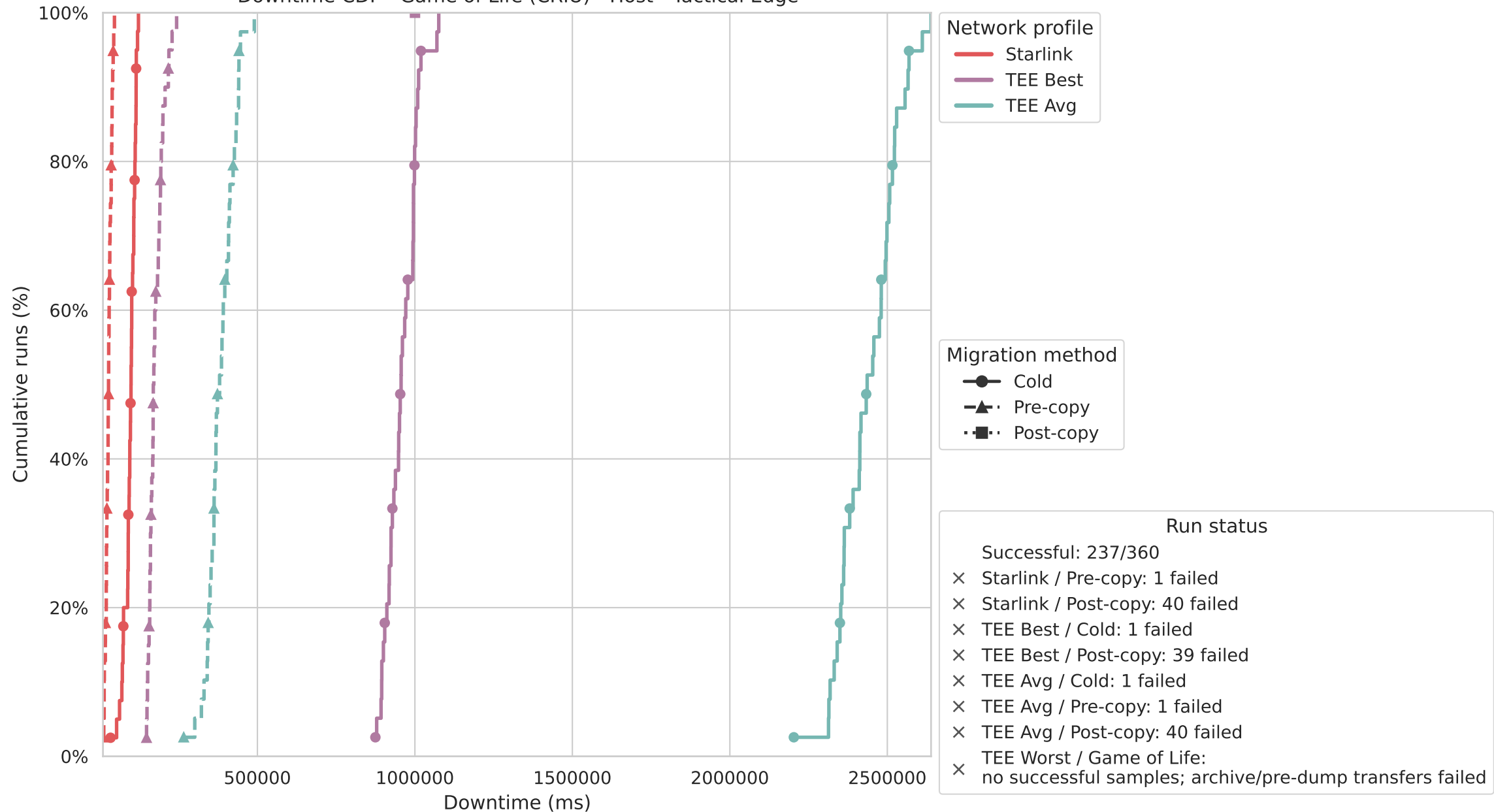
Downtime CDF - Game of Life (CRIU) - Host - Tactical Edge
