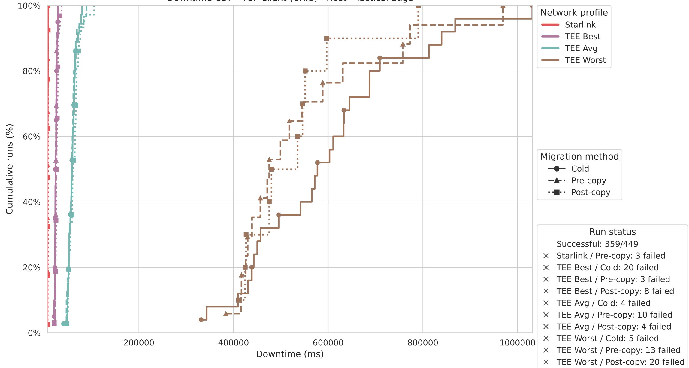
Downtime CDF - TCP Client (CRIU) - Host - Tactical Edge
