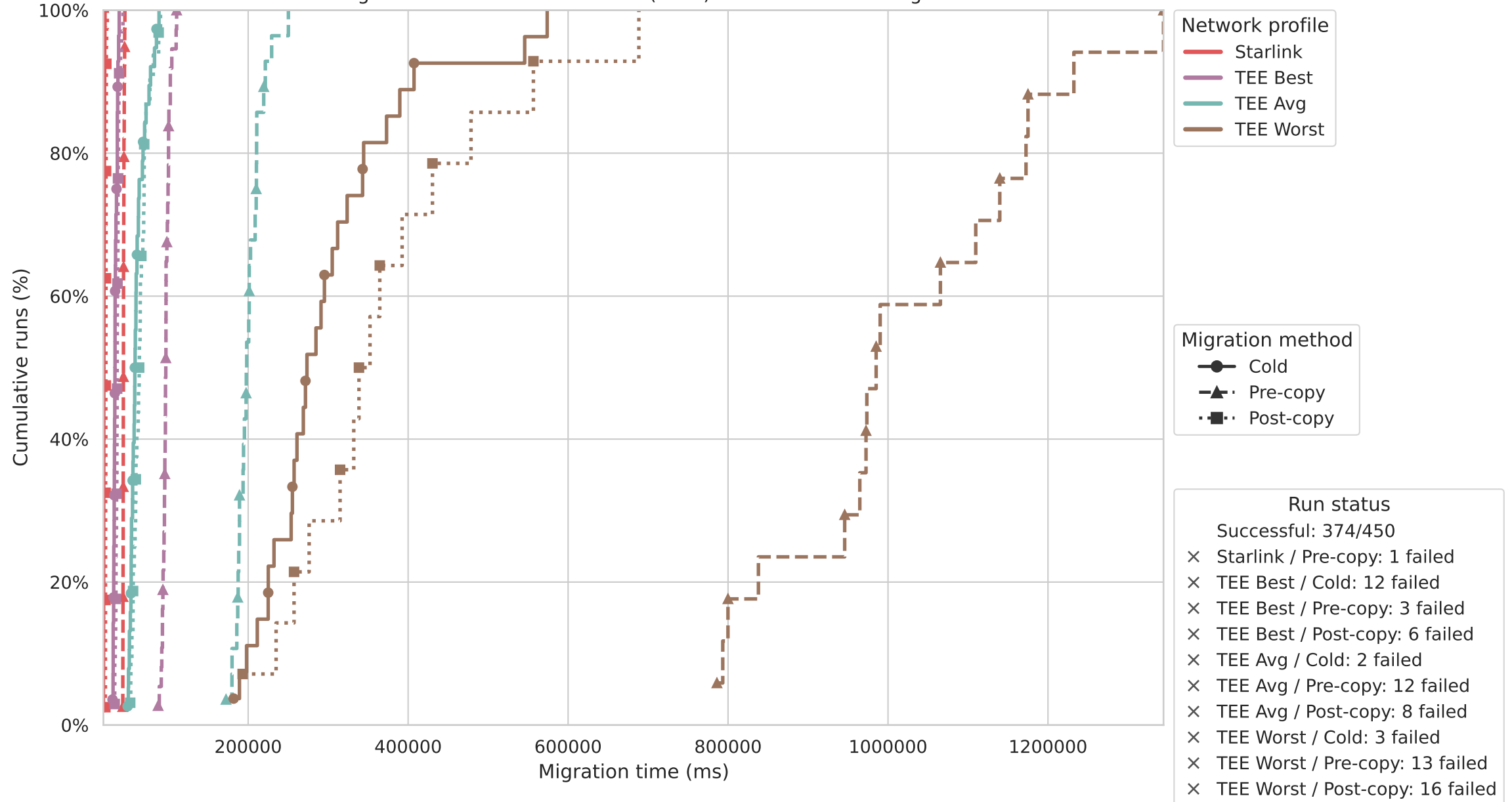
Migration Time CDF - TCP Client (CRIU) - Direct - Tactical Edge
