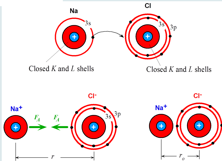
Fig: formation of ionic bond between Na and Cl
