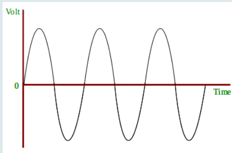
Fig: Alternating Current (AC) Current (DC)
