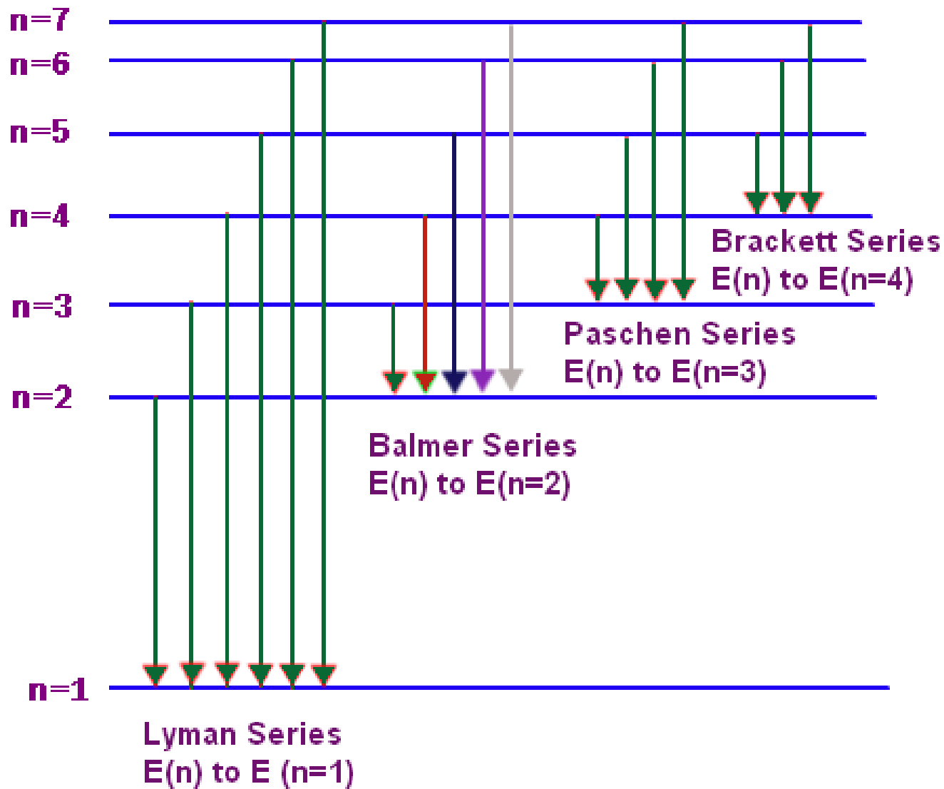
Fig: Atomic Energy Level (Spectra)
