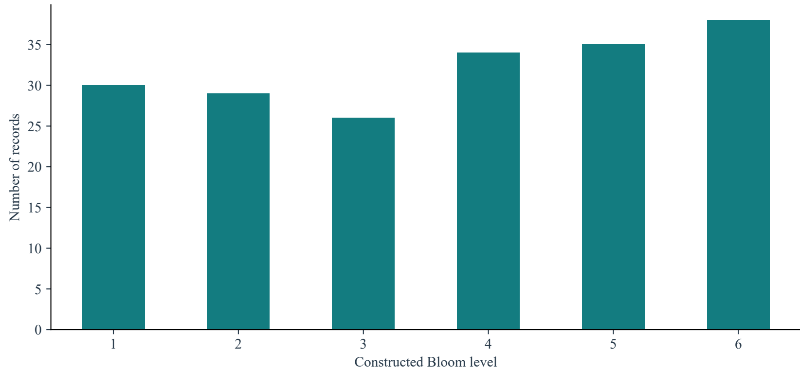
Synthetic records: level distribution
