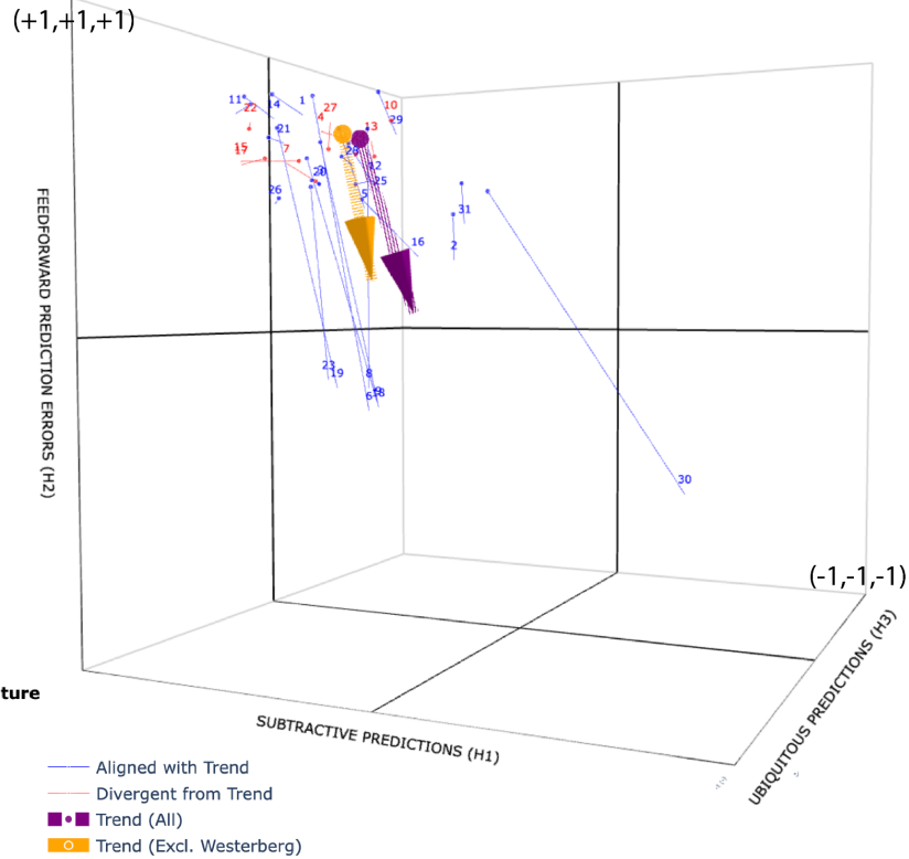
Figure 8: Three-Dimensional vectors of each paper from the Local to the Global oddball position. Each paper's vector is shown independently. The average movement (vector direction) without the outlier study (Westerberg, Xiong, et al., & Xiong, 2025) is shown in yellow, and the average movement of all studies is shown in purple. Individual study's vectors are labeled as blue if their individual vector was aligned to the Westerberg, Xiong, et al., & Xiong (2025) study's vector on all three axes, and red otherwise.
