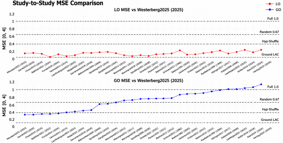
Figure 6: Mean squared error values measuring the distance between each paper and the outlier paper (Westerberg et al. & Xiong, 2025), separately for the local oddball (upper subpanel) and global oddball (lower subpanel) contexts. Papers are ordered from left to right in order of increasing global-oddball MSD to Westerberg et al. & Xiong (2025).
