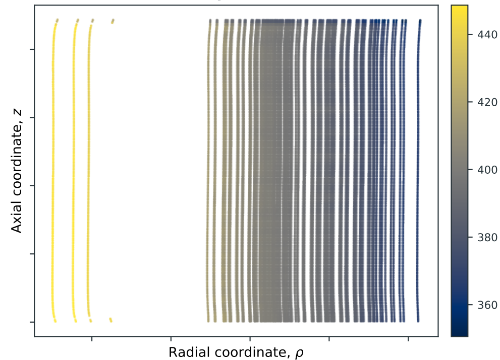
Maximum principal stress
