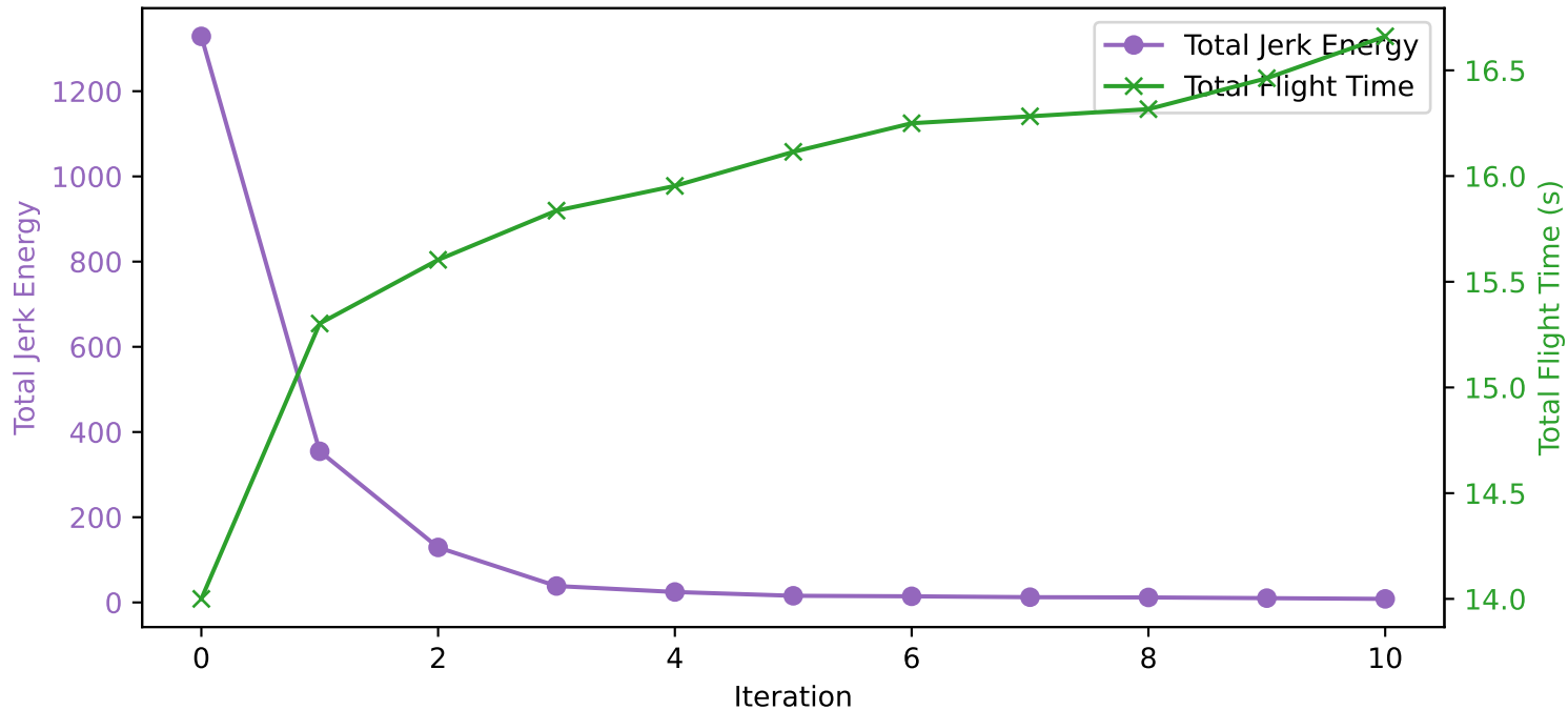
MINCO Iteration History: Jerk Energy & Flight Time
