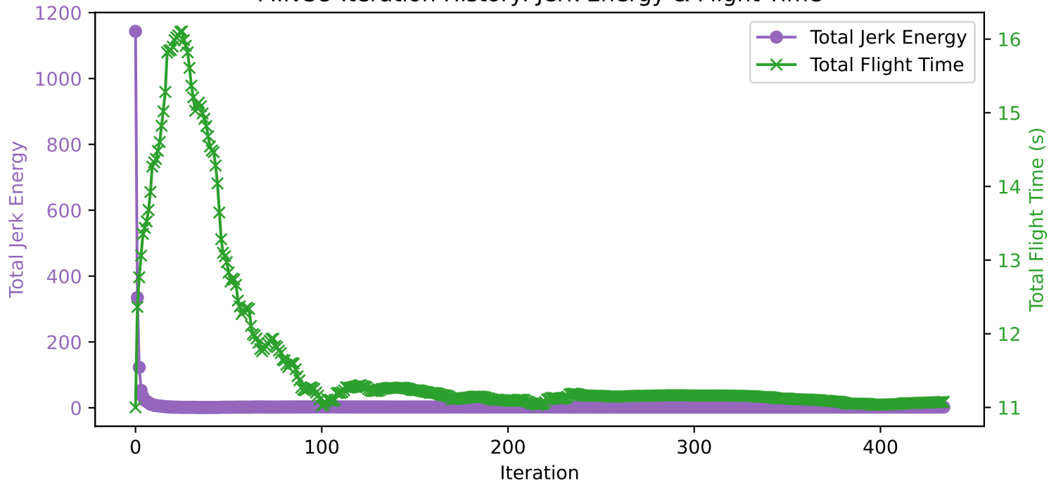
MINCO Iteration History: Jerk Energy & Flight Time
