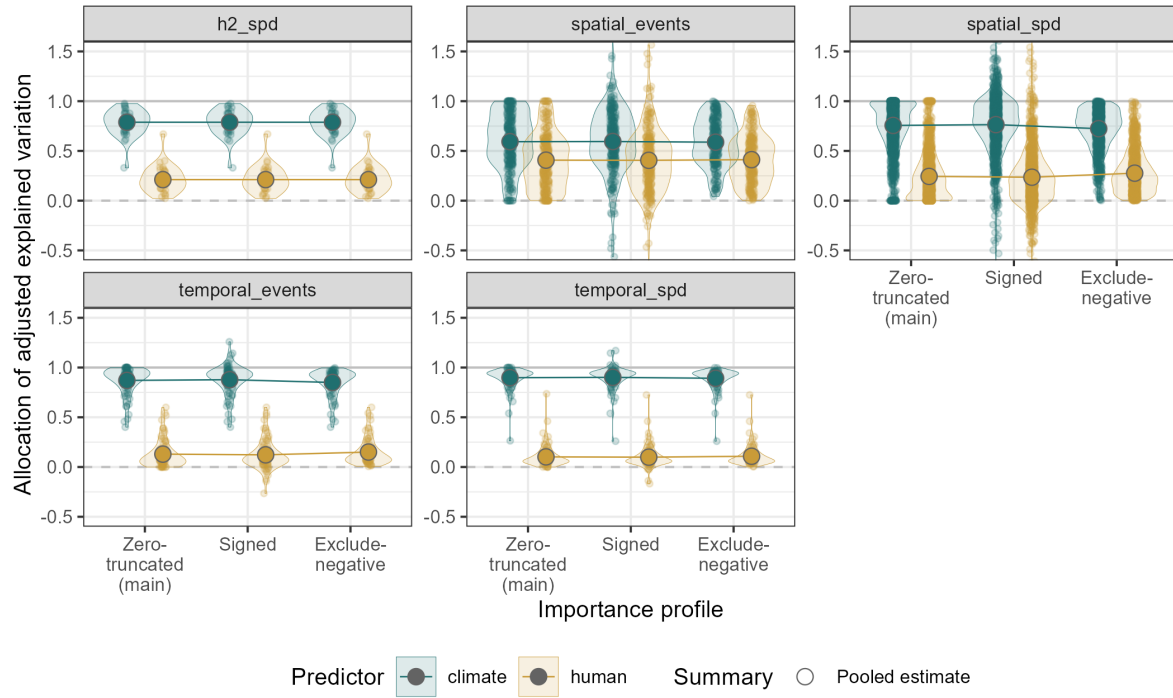
Figure 1: Zero-truncated main-figure allocation and two sensitivity profiles, calculated from the preserved fitted HVarPart results.
