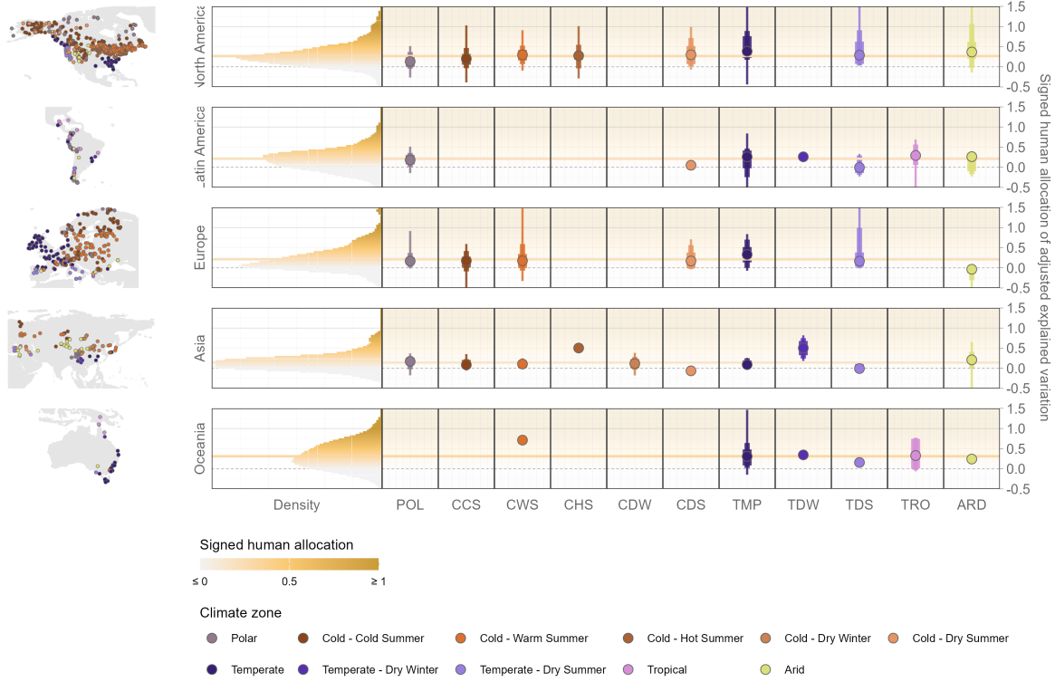
Supplementary signed Figure 2. Unmodified signed human allocation, displayed from -0.5 to 1.5; all values are retained in the source table.
