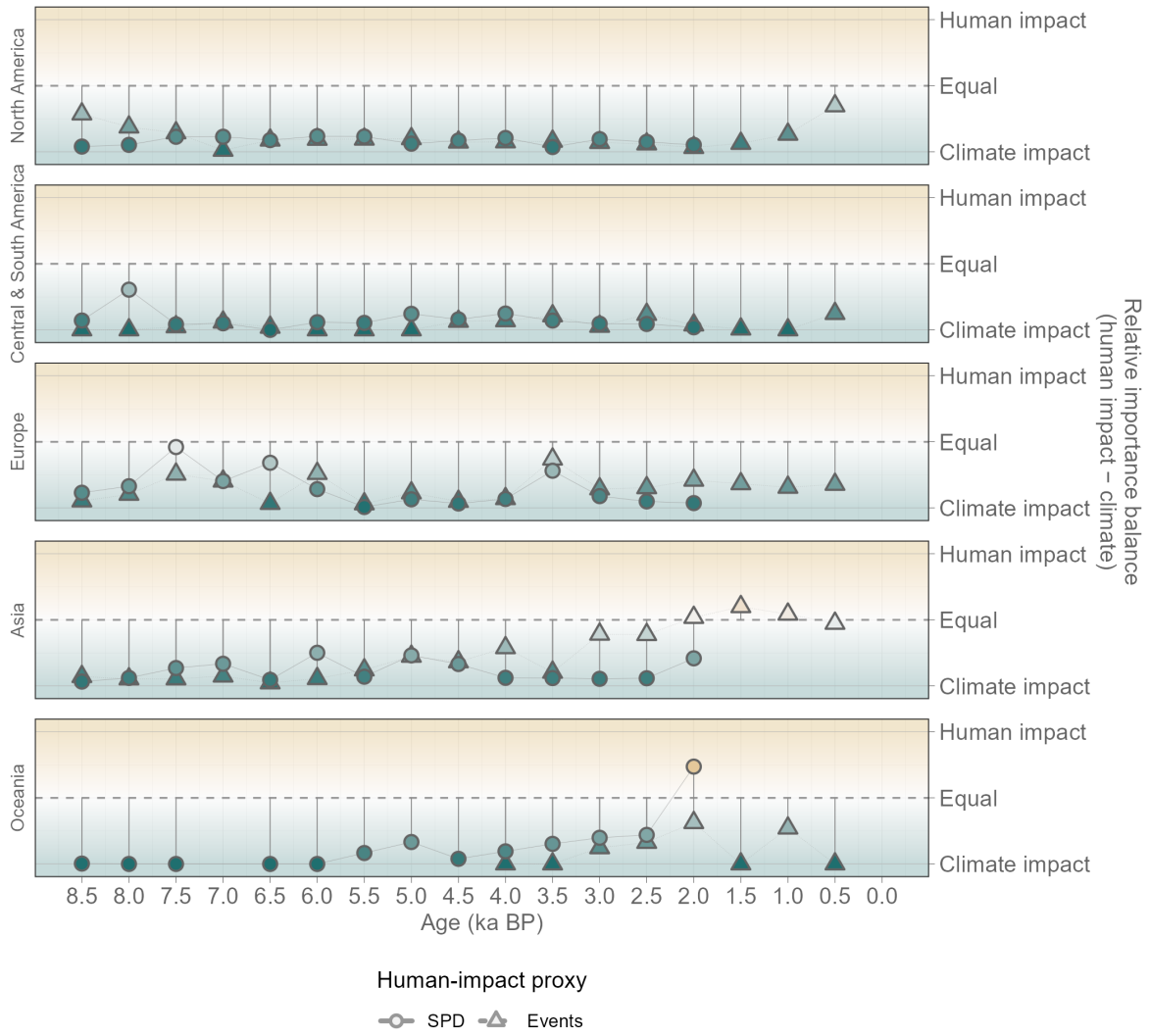
Revised main manuscript Figure 3. Temporal balance between zero-truncated human and climate allocations.
