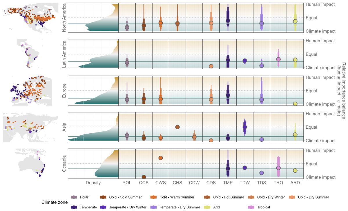
Revised main manuscript Figure 2. Spatial balance between zero-truncated human and climate allocations.
