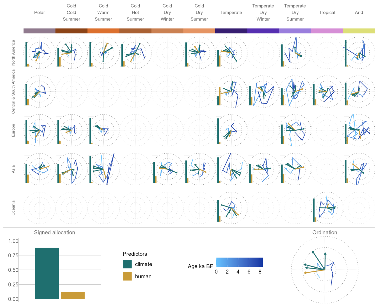
Supplementary signed Figure 4. Multidimensional community-change ordinations with separate unmodified signed human and climate allocations.
