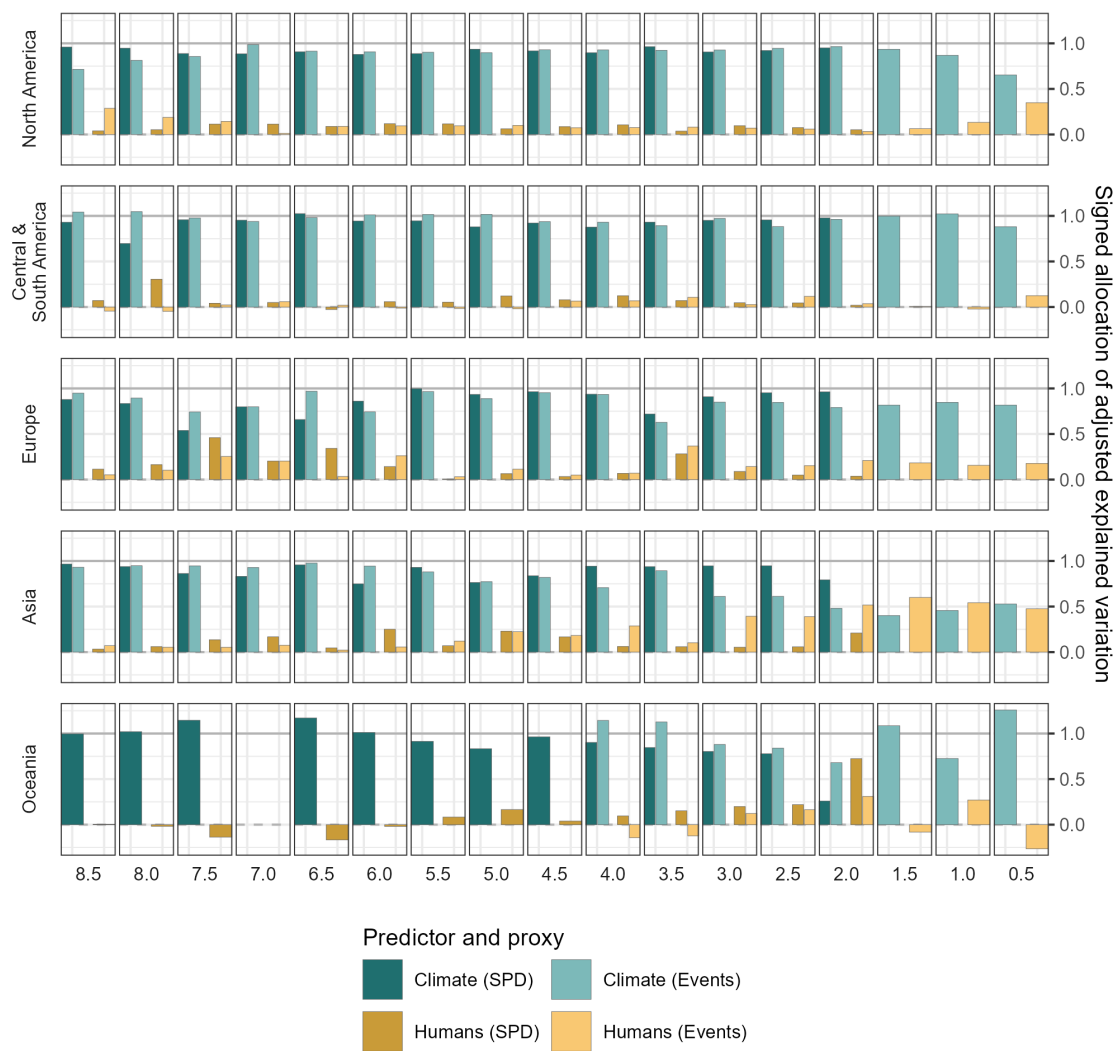
Supplementary signed Figure 3. Unmodified signed climate and human allocations through time.
