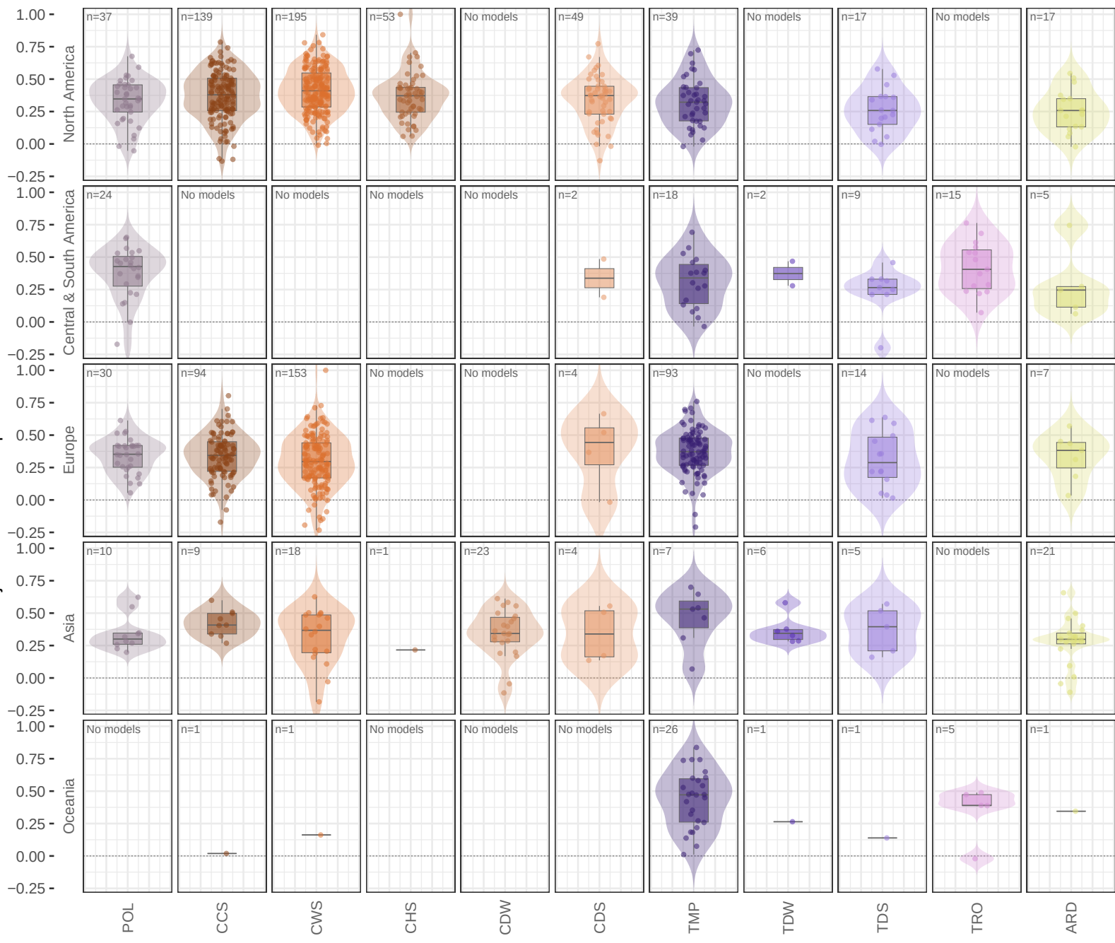
Adjusted R^2 across spatial SPD models
