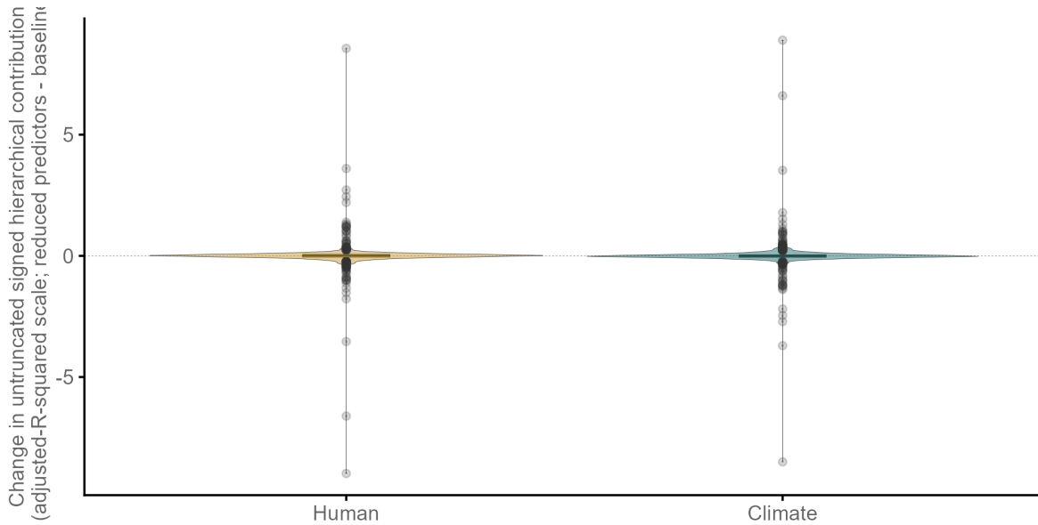
Figure 2: Sensitivity of untruncated signed hierarchical contributions after reducing collinear PAP responses. This is a supplementary decomposition diagnostic; missing values are retained as missing.
