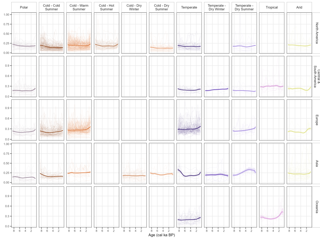
Supplementary Fig. S18 (reproduced). Rate of compositional change. Regional trajectories over the observed sequence coverage.
