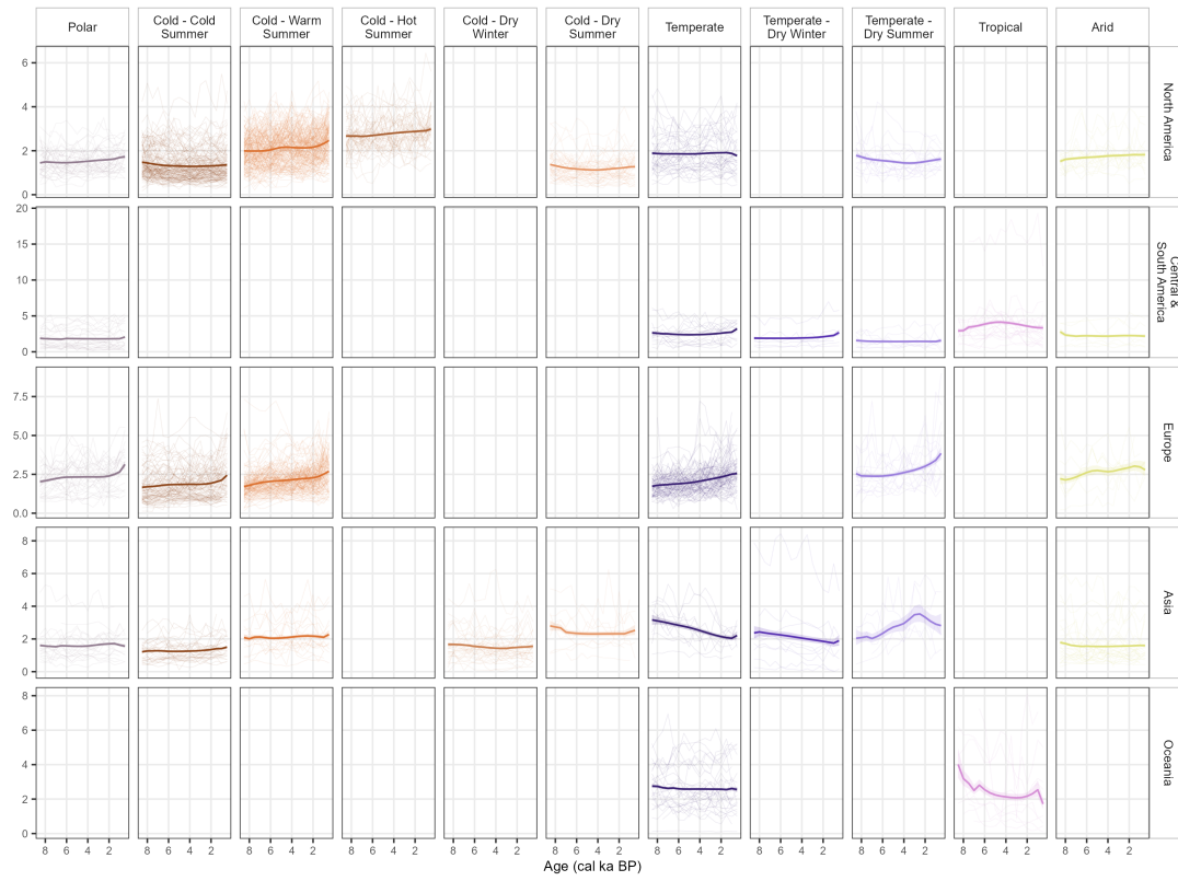
Supplementary Fig. S15 (reproduced). Shannon–Simpson diversity difference ( N_1 - N_2 ). Regional trajectories over the observed sequence coverage.
