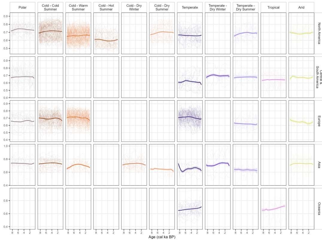
Supplementary Fig. S16 (reproduced). Simpson-to-Shannon diversity ratio ( N_2/N_1 ). Regional trajectories over the observed sequence coverage.
