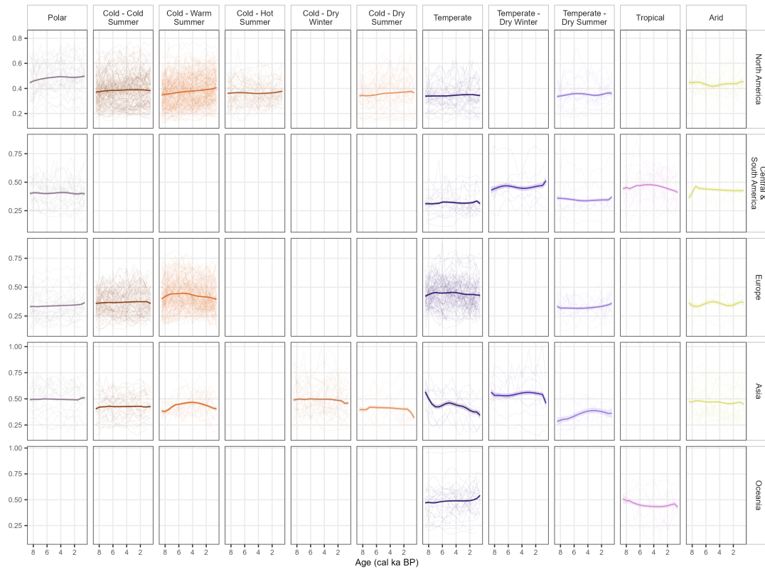
Supplementary Fig. S17 (reproduced). Shannon-diversity-to-richness ratio ( N_1/N_0 ). Regional trajectories over the observed sequence coverage.
