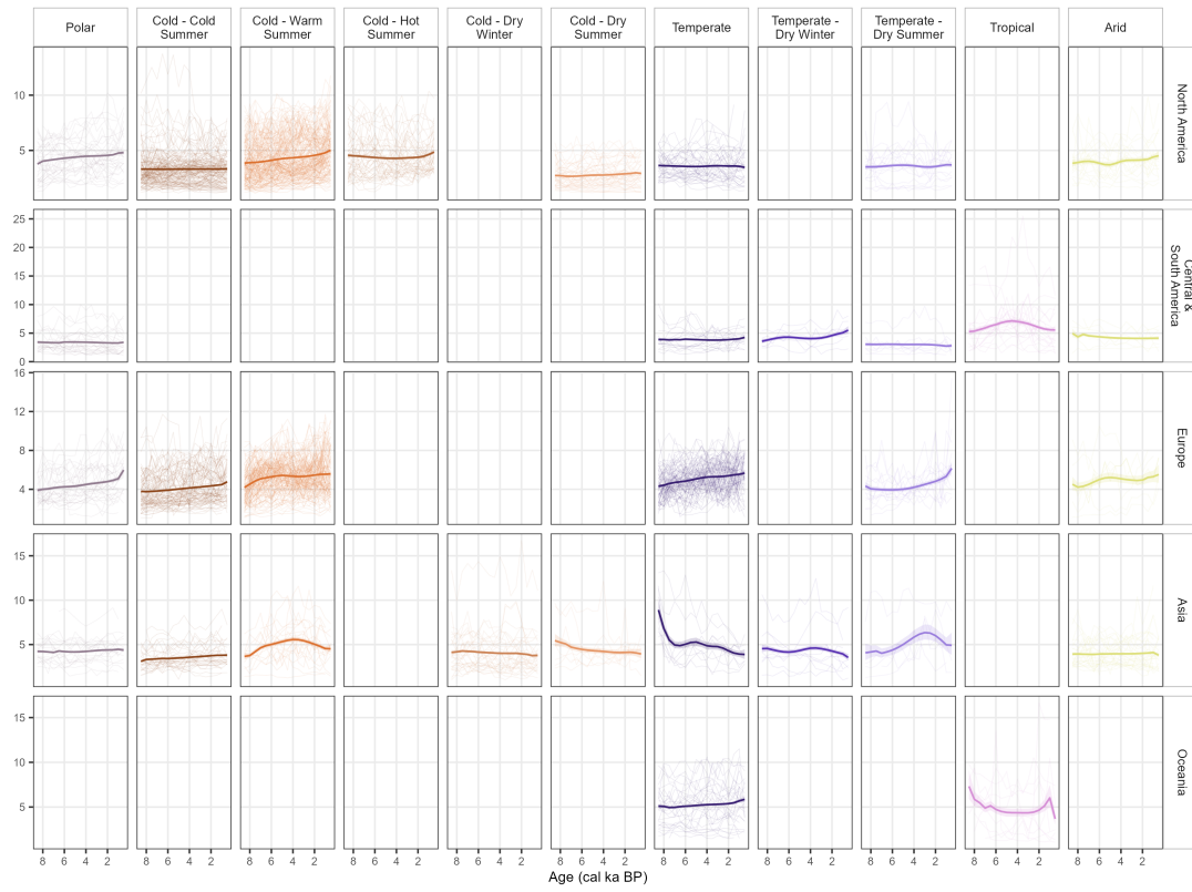
Supplementary Fig. S14 (reproduced). Simpson-effective diversity ( N_2 ). Regional trajectories over the observed sequence coverage.
