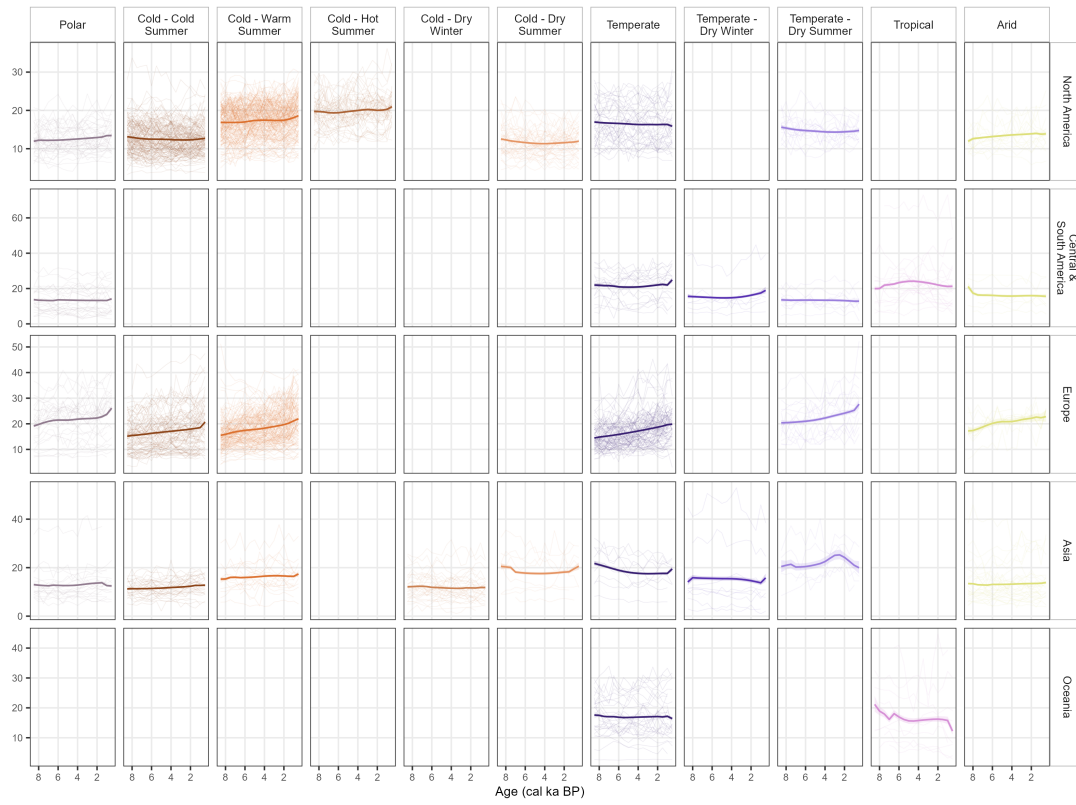
Supplementary Fig. S12 (reproduced). Taxonomic richness ( N_0 ). Regional trajectories over the observed sequence coverage.
