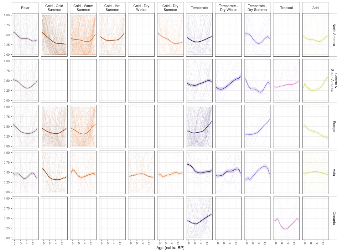
Supplementary Fig. S20 (reproduced). Diversity change-point density. Regional trajectories over the observed sequence coverage.
