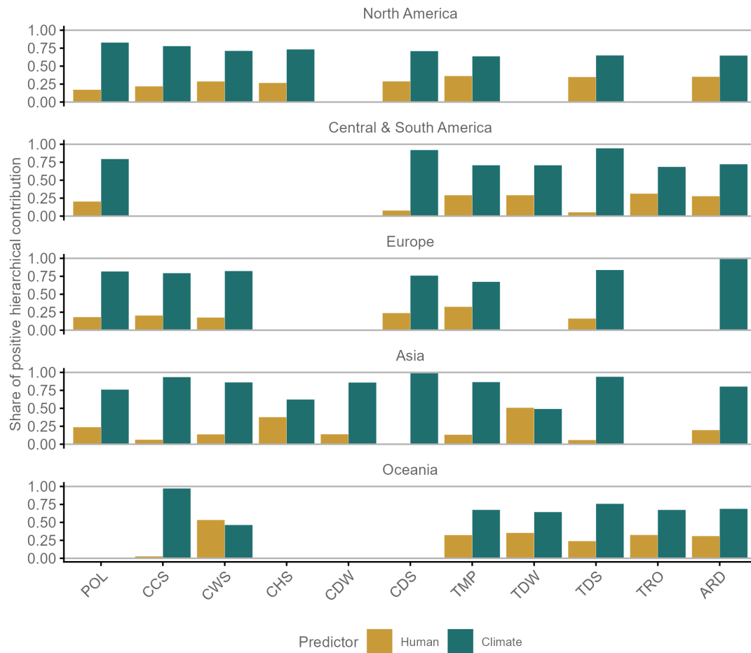
Supplementary Fig. S30 (reproduced). Climate–human allocation with a reduced PAP response. The spatial H1 analysis was repeated with a less redundant set of PAPs. This zero-truncated display favours climate in most regional groups; the matched signed comparison is reported above and in Supplementary Table S7.
