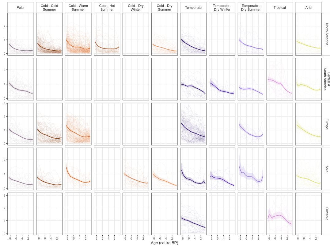
Supplementary Fig. S19 (reproduced). DCCA axis 1. Regional trajectories along the primary compositional gradient; the axis sign is arbitrary.
