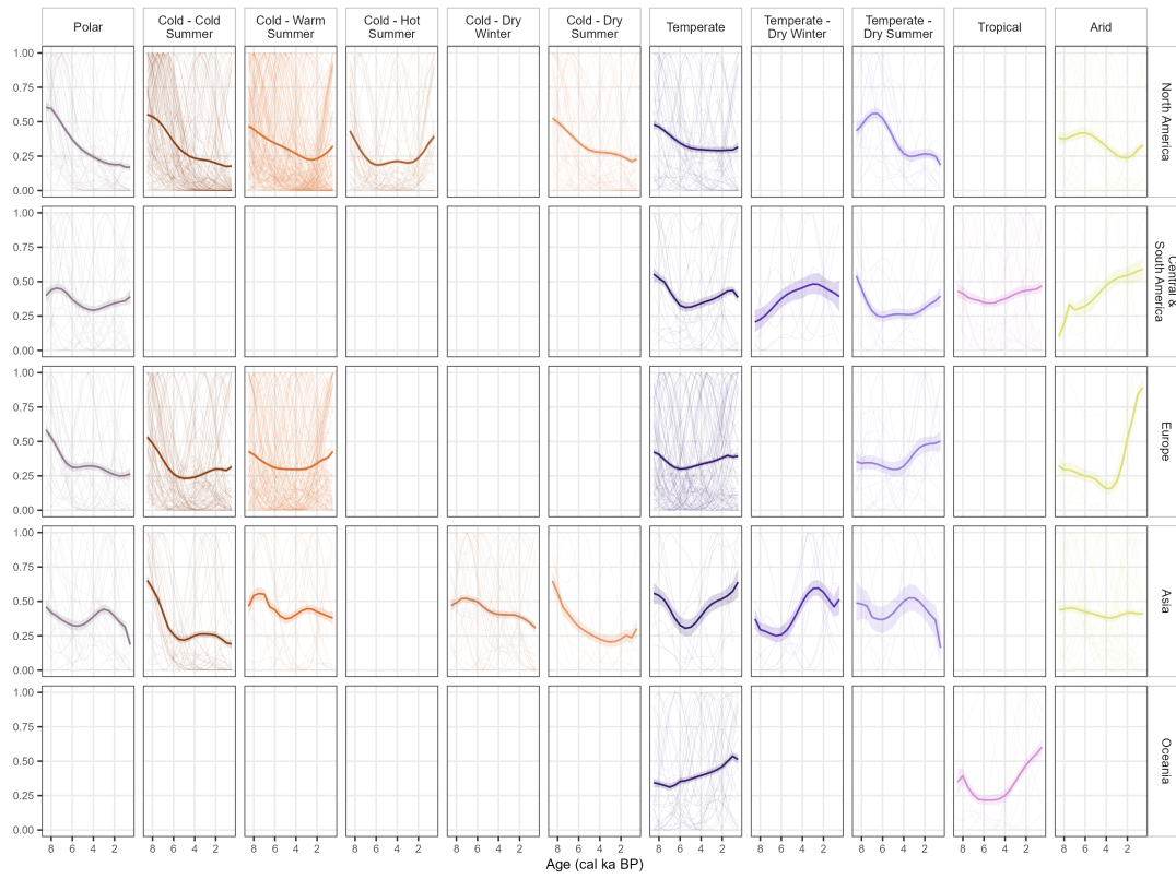
Supplementary Fig. S21 (reproduced). Turnover change-point density. Regional trajectories over the observed sequence coverage.
