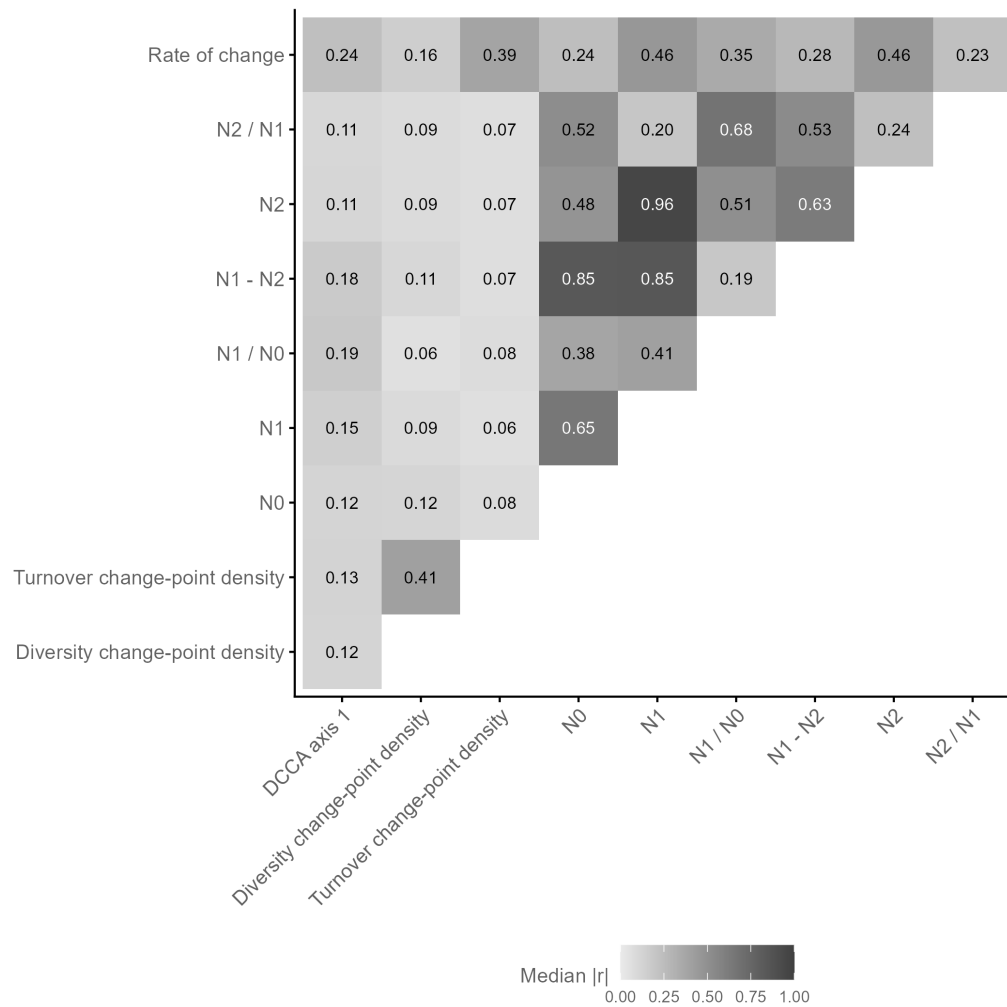
Supplementary Fig. S24 (reproduced). Correlations among pollen assemblage properties. Tiles give the median absolute pairwise correlation across eligible continental-group-region subsets. They show the strength, not the direction, of association.
