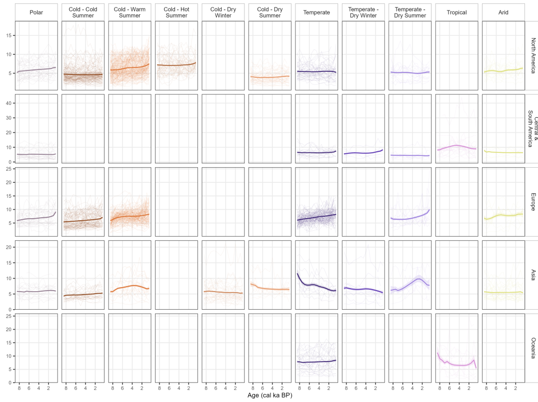
Supplementary Fig. S13 (reproduced). Shannon-effective diversity ( N_1 ). Regional trajectories over the observed sequence coverage.
