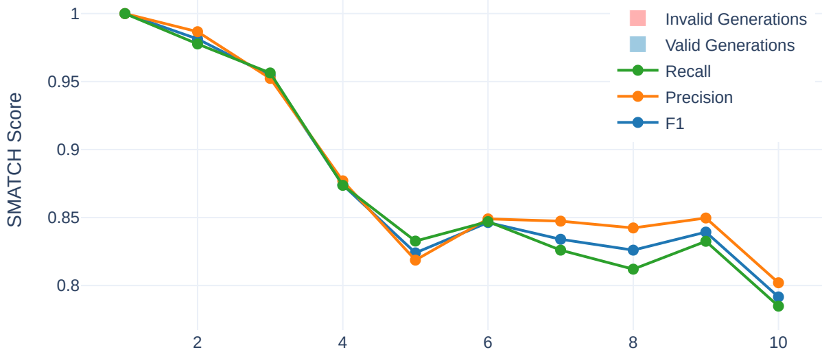
SMATCH Scores by AMR Depth
