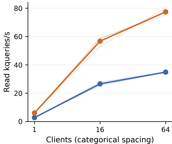
Telemetry | SQLite native
