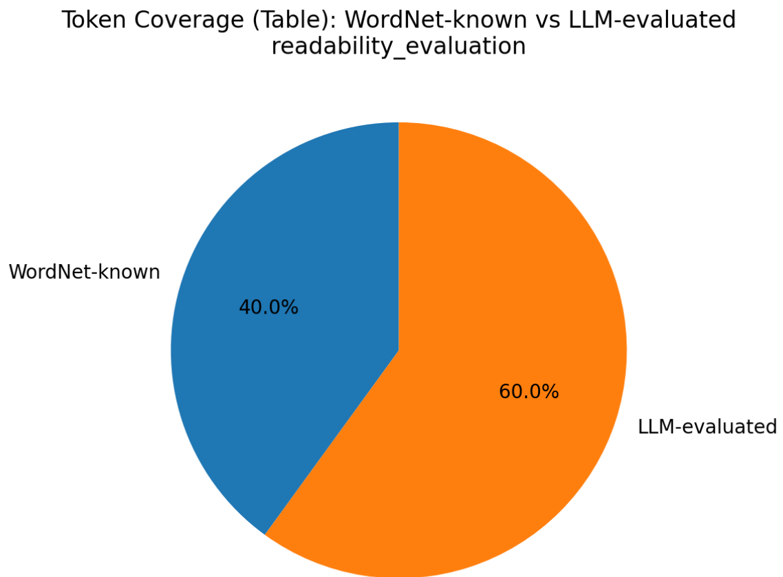
Figure 3. Token Coverage at Table Level. Pie chart shows the share of tokens handled by WordNet vs tokens requiring LLM evaluation.
