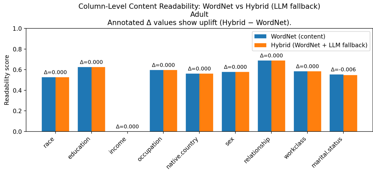
Figure 2. Column-Level Content Readability (WordNet vs Hybrid). Bars compare WordNet-only vs Hybrid (WordNet+LLM fallback) per column. Annotated \Delta values represent uplift (Hybrid – WordNet) per column.
