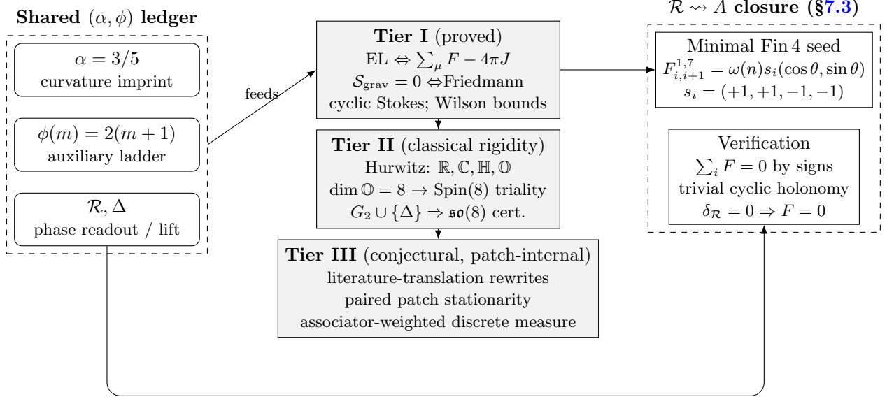
FIGURE 1. Executive summary. The shared (\alpha, \phi) ledger forced by the predecessor papers feeds both the proved Tier-I dynamics (EL identity, Friedmann constraint, holonomy bounds) and the explicit minimal-cycle realization \mathcal{R} \rightsquigarrow A . Tier II is classical division-algebra rigidity plus the certified G_2 \cup \{\Delta\} \Rightarrow \mathfrak{so}(8) closure; Tier III is a patch-internal interoperability programme (literature-translation rewrites, paired patch stationarity, associator-weighted discrete measure)— not a continuum-limit programme. Per the patch-theory reader contract above, no continuum limit is required for foundational validity.
