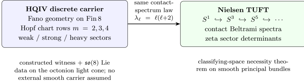
FIGURE 2. Discrete Hopf-shell chart on the octonion carrier (left) and Nielsen’s nested Hopf fibration (right) carry the same contact-spectrum law; methodology differs (witness vs classification). The nested fibration is finite at the division-algebra ceiling (§2.1).
