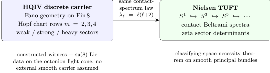
FIGURE 2. Discrete Hopf-shell chart on the octonion carrier (left) and Nielsen’s nested Hopf fibration (right) carry the same contact-spectrum law; methodology differs (witness vs classification).
