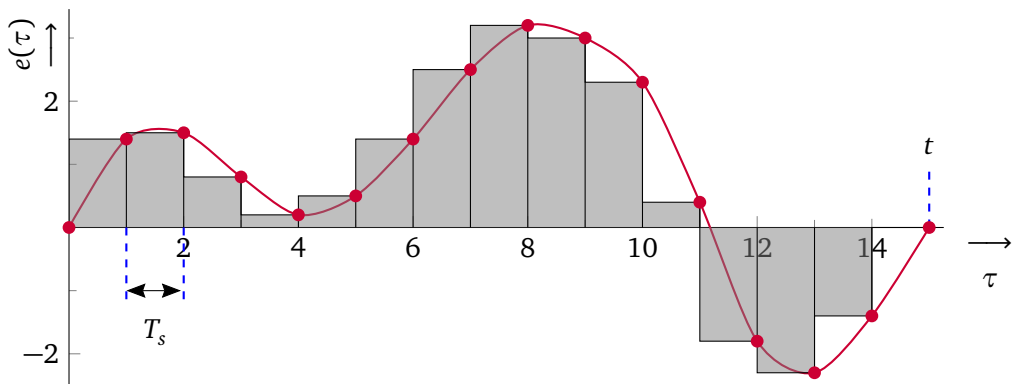
Figuur 2.3: Backward Rectangular Method (BRM).
