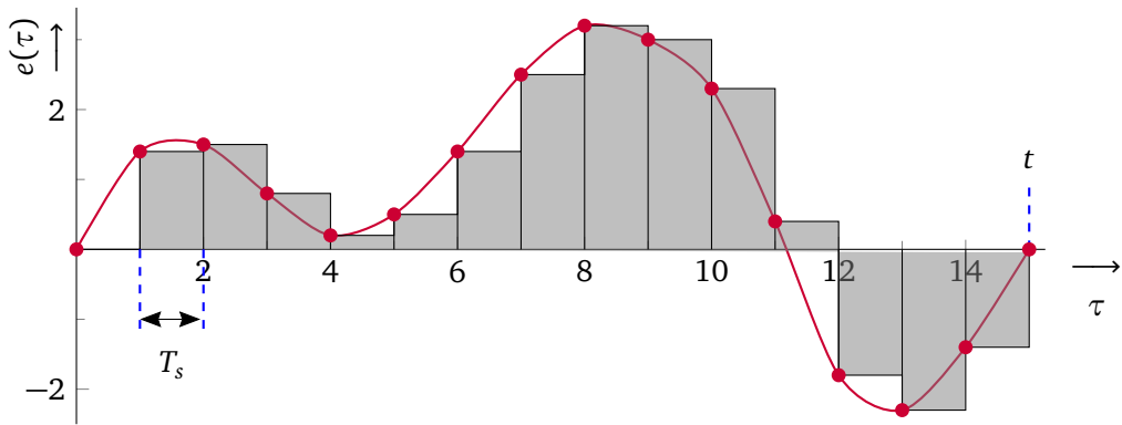
Figuur 2.2: Forward Rectangular Method (FRM).
